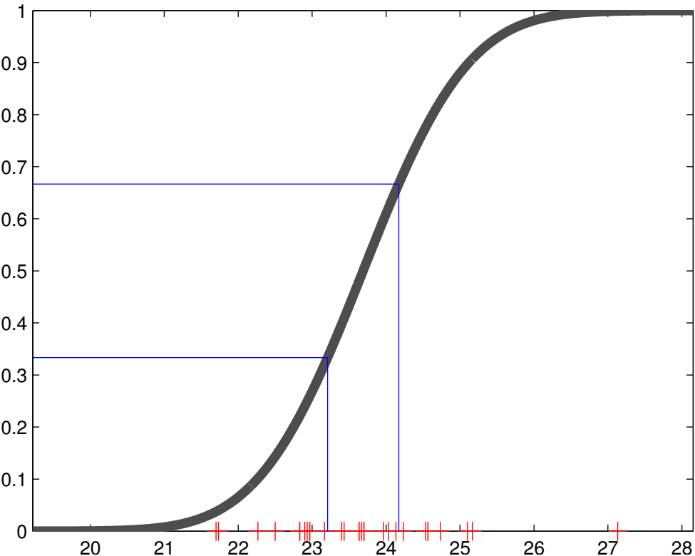
JJA temperature in Trieste CDF (1980–2009)
