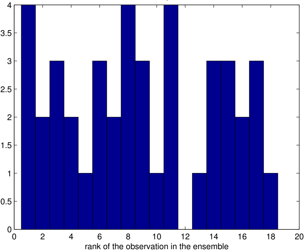
rank histogram
