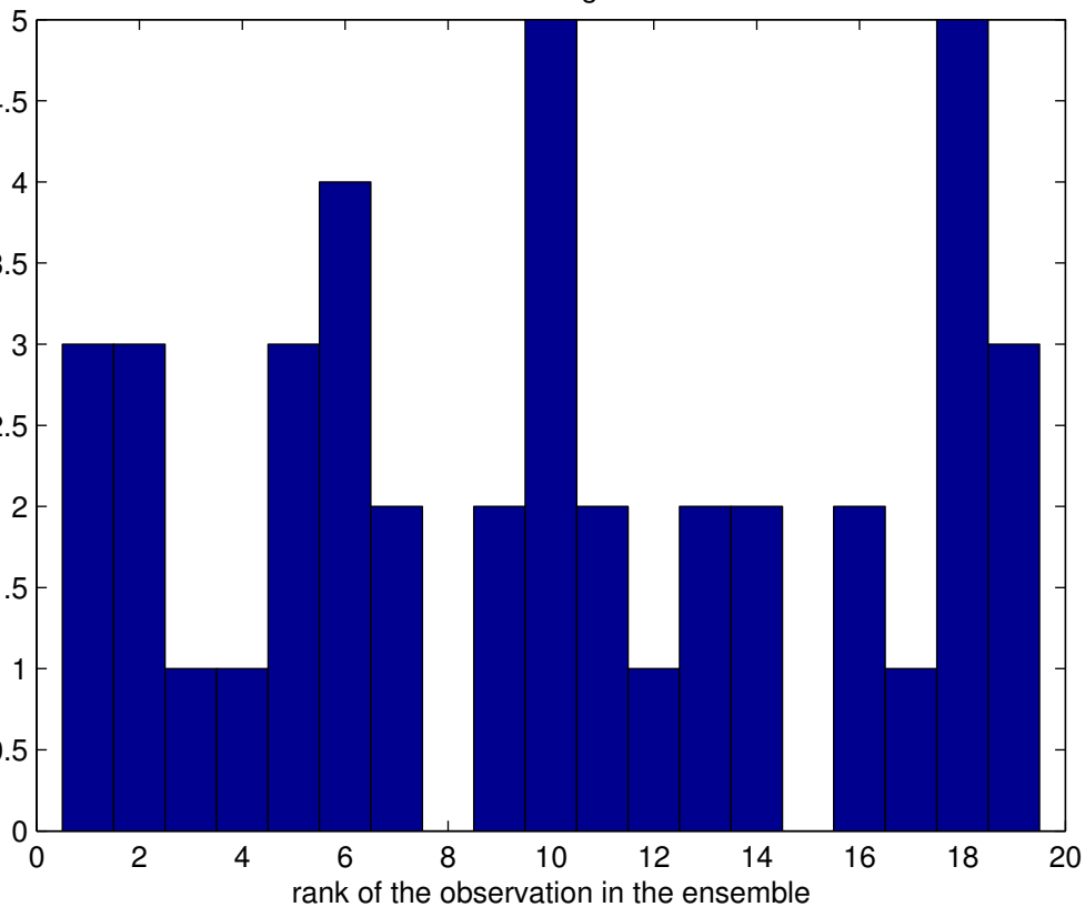
rank histogram
