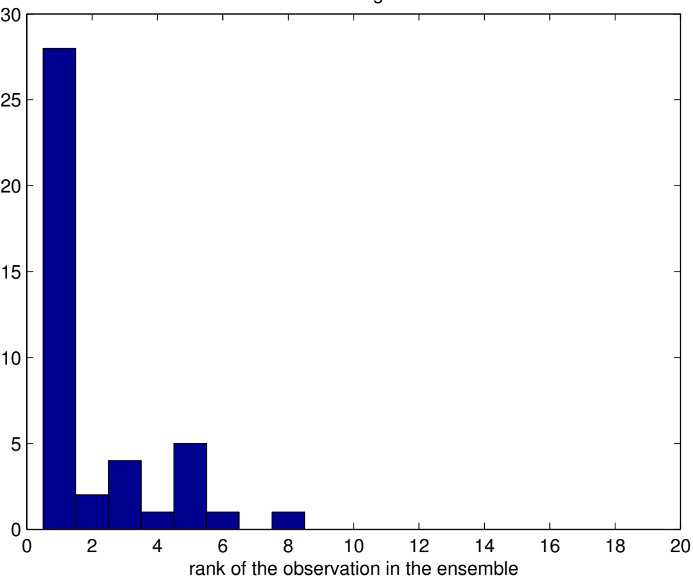
rank histogram
