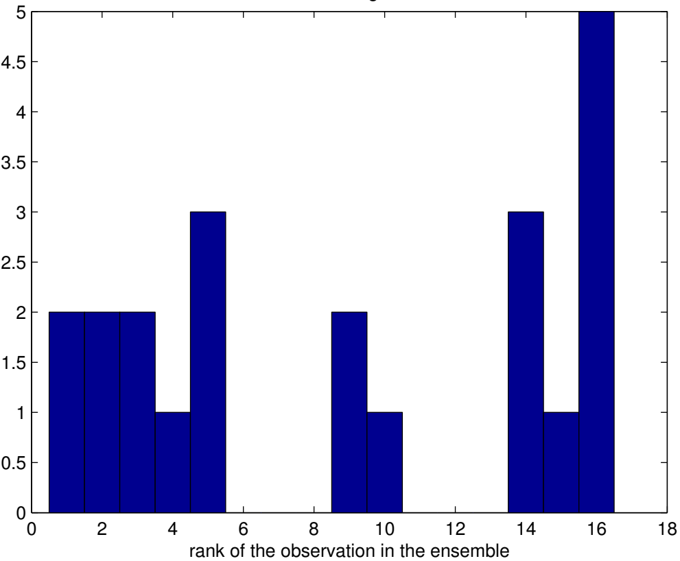
rank histogram
