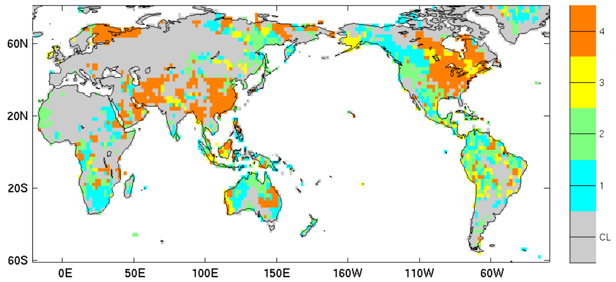
Cross-validation
