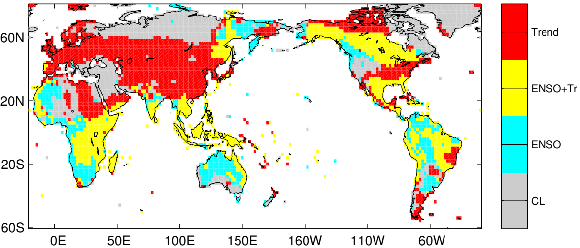
corrected AIC
