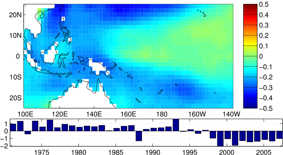
EOF 2 variance explained =16%
