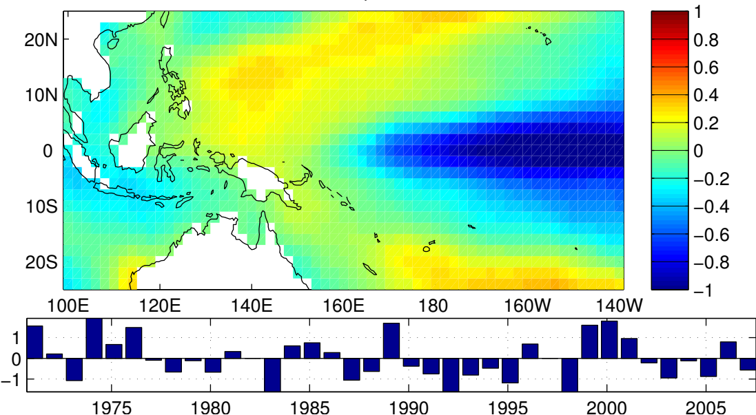
EOF 1 variance explained =50%
