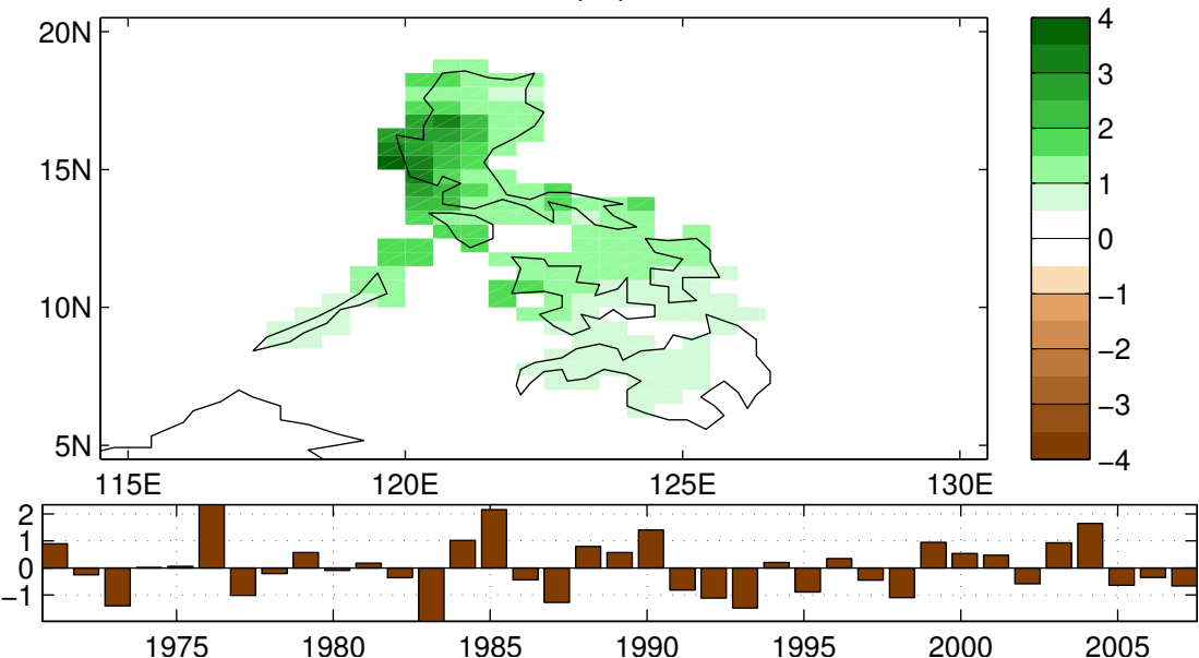
EOF 1 of prcp
