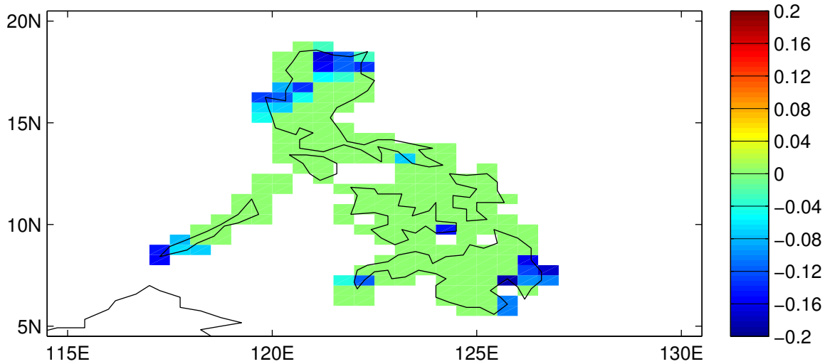
Change in 1-error var/clim var
