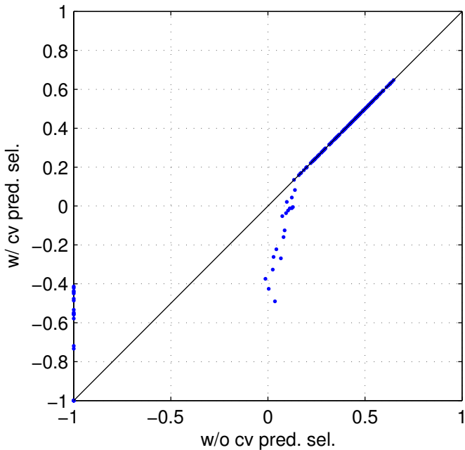
correlation
