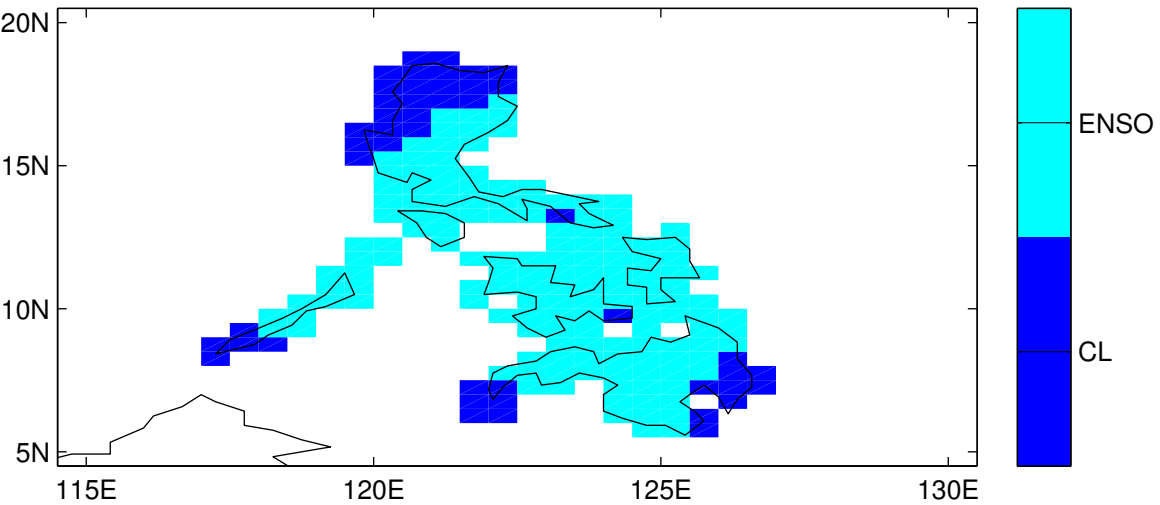
min AIC selected model
