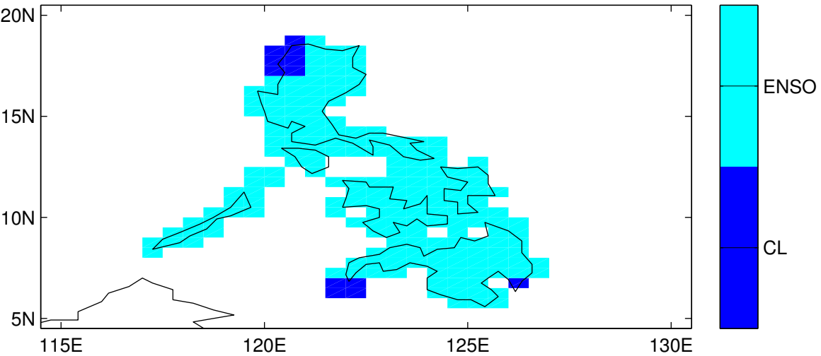
max AIC selected model
