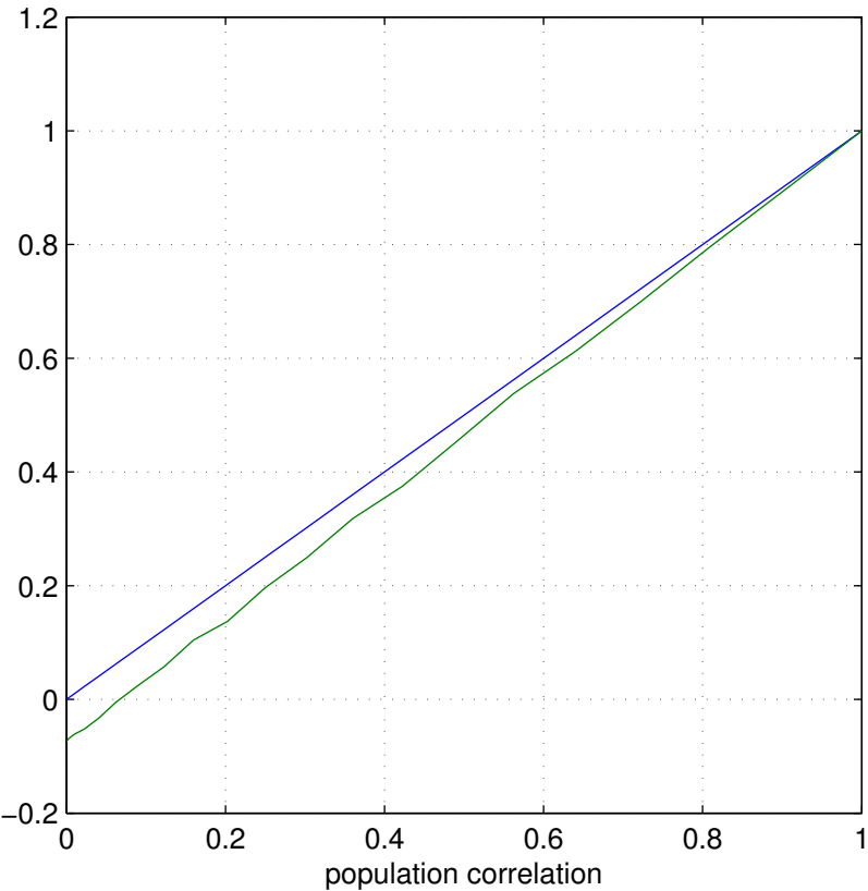
cv 1 – normalized error variance
