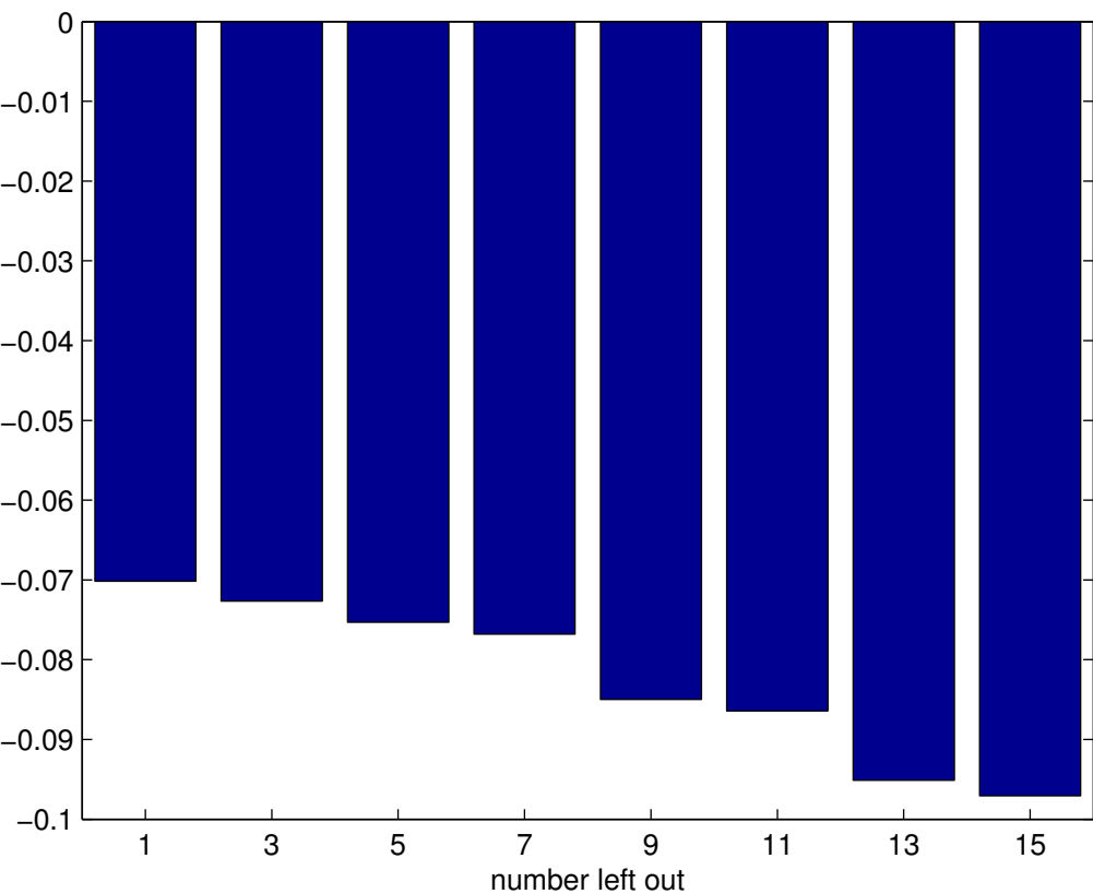
cross-validated 1-normalized error variance
