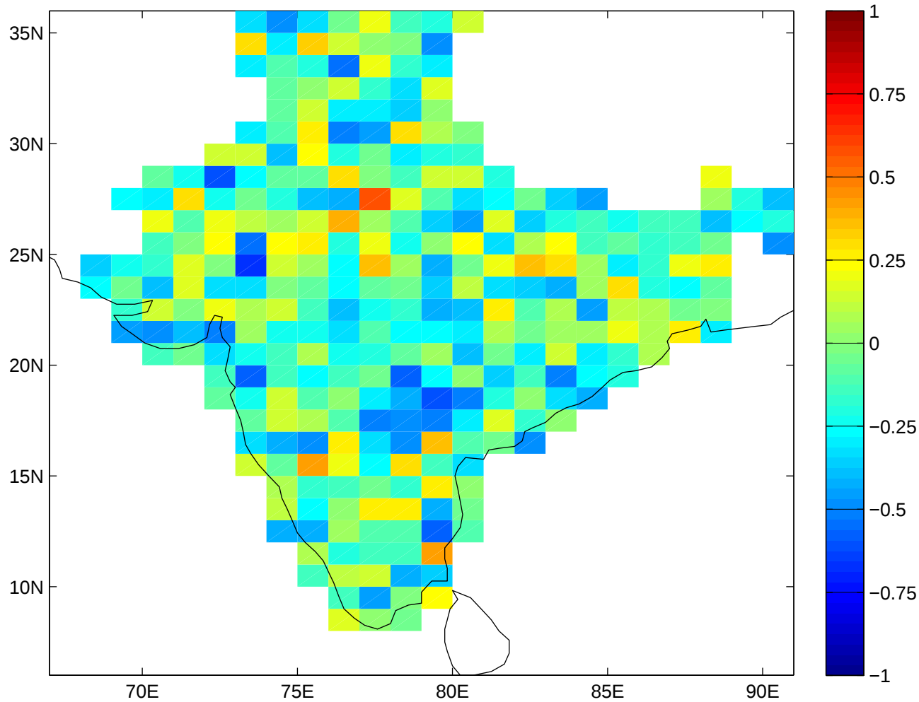
ECHAM4.5 CA g=-0.12 rms=8.1
