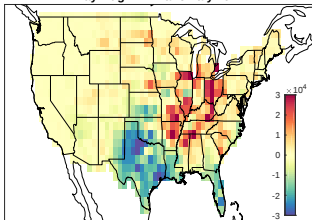
May-Aug NLDN anomaly 2011
