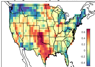
May-Aug PRCP and May-Aug PDO 2003-2016
