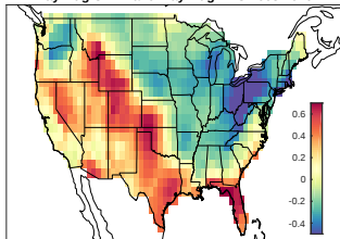
May-Aug CAPE and May-Aug PDO 2003-2016
