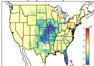
May-Aug NLDN anomaly 2012
