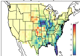
May-Aug NLDN anomaly 2013
