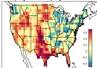
May-Aug NLDN and May-Aug PDO 2003-2016
