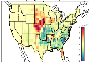
May-Aug NLDN anomaly 2014
