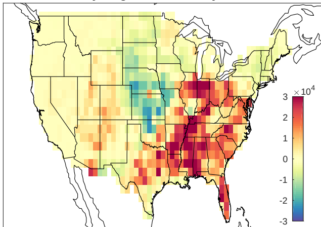
May-Aug NLDN anomaly 2003
