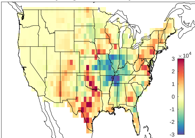
May-Aug NLDN anomaly 2007
