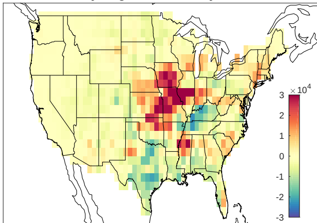
May-Aug NLDN anomaly 2008
