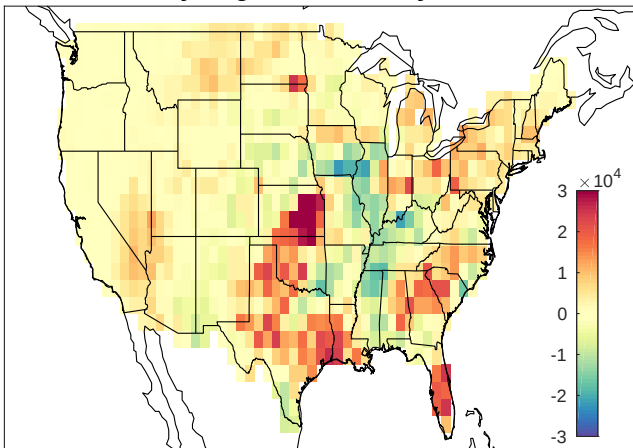
May-Aug NLDN anomaly 2005
