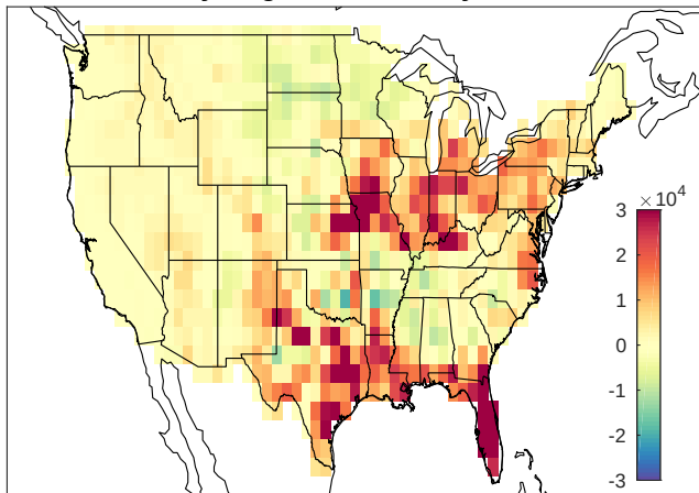
May-Aug NLDN anomaly 2004
