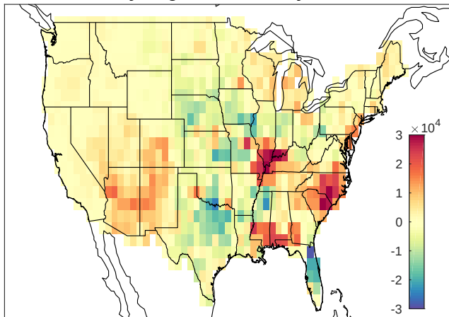
May-Aug NLDN anomaly 2006
