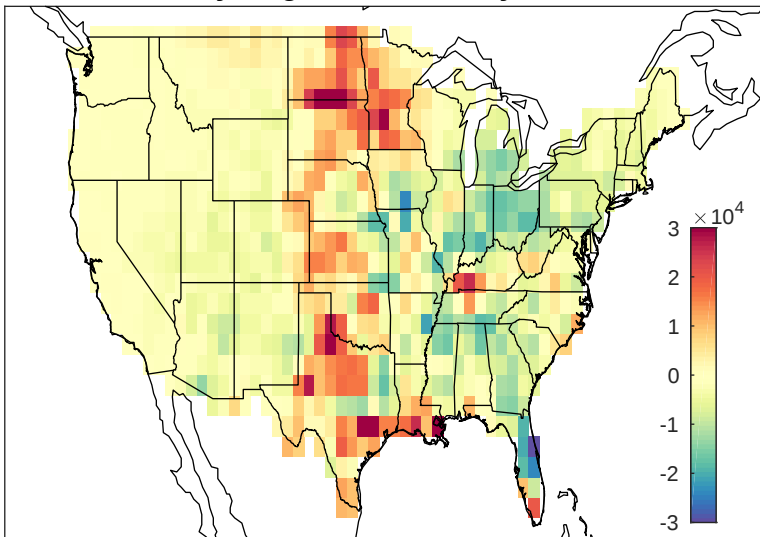
May-Aug NLDN anomaly 2016
