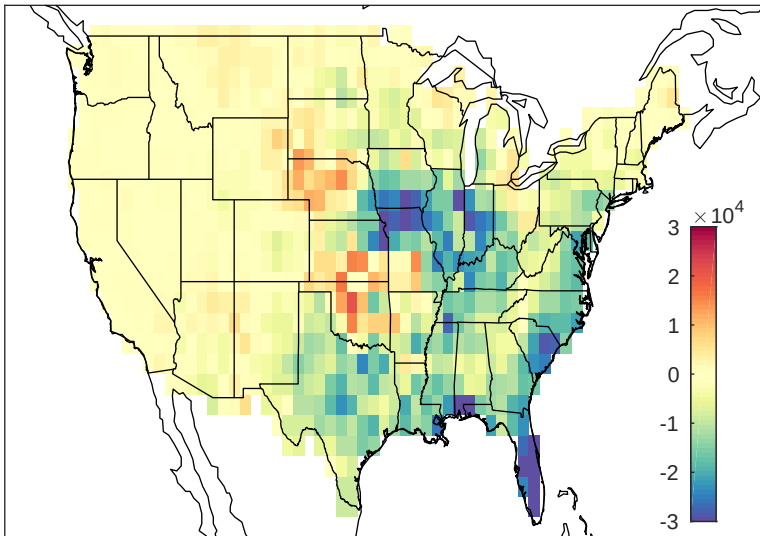
May-Aug NLDN anomaly 2013
