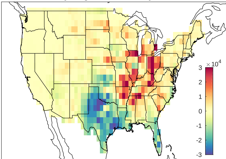
May-Aug NLDN anomaly 2011
