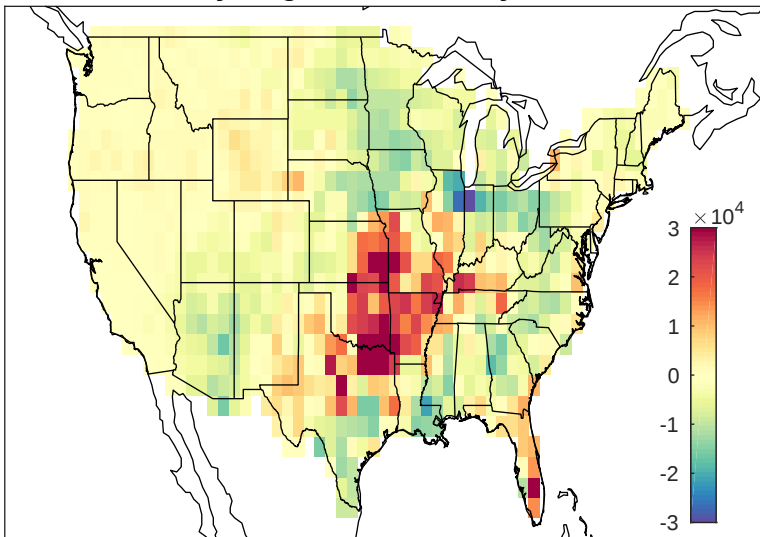
May-Aug NLDN anomaly 2009
