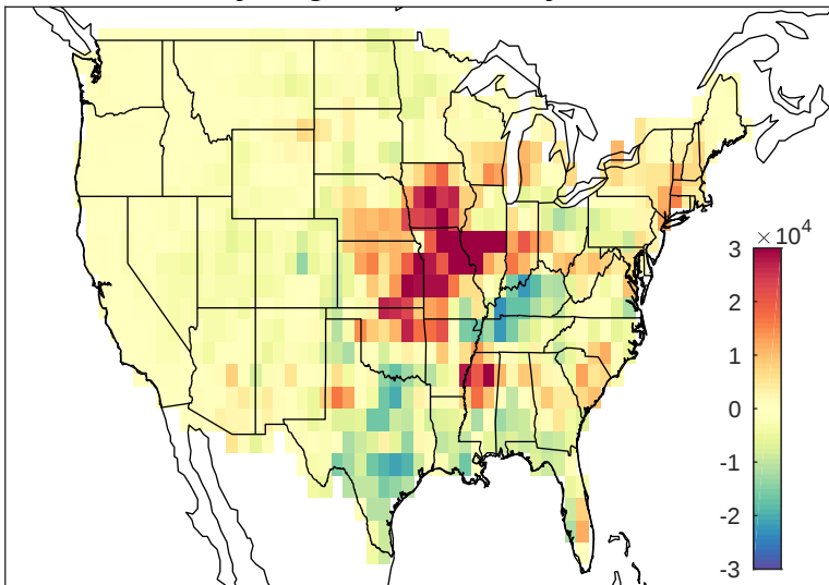
May-Aug NLDN anomaly 2008
