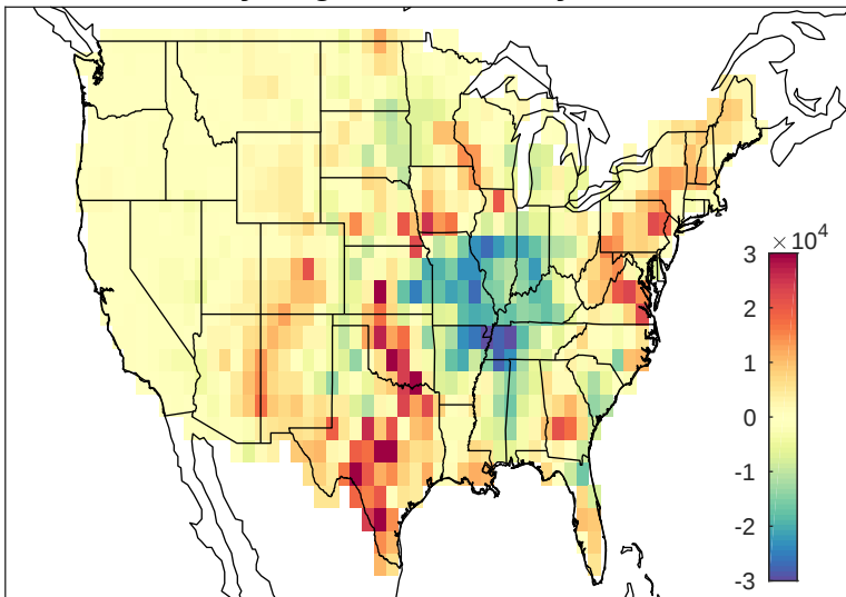
May-Aug NLDN anomaly 2007
