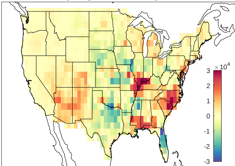
May-Aug NLDN anomaly 2006
