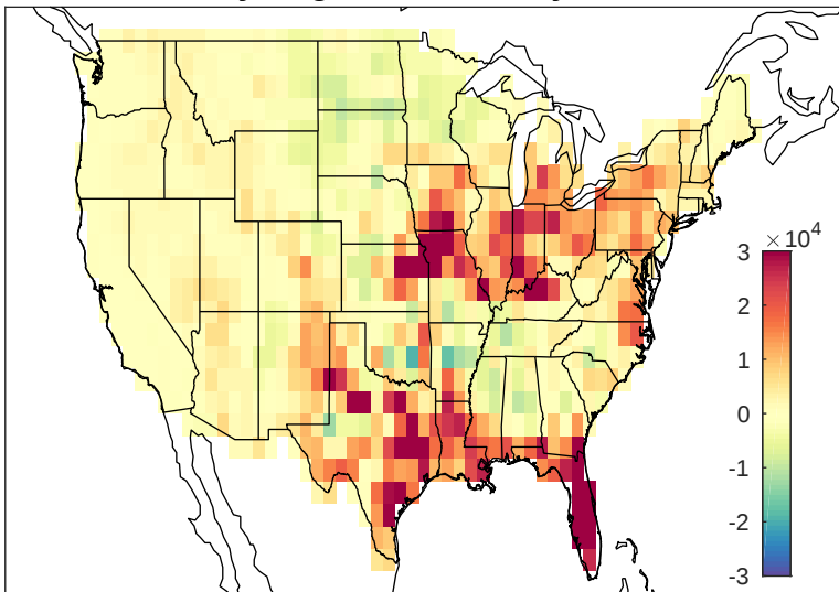
May-Aug NLDN anomaly 2004
