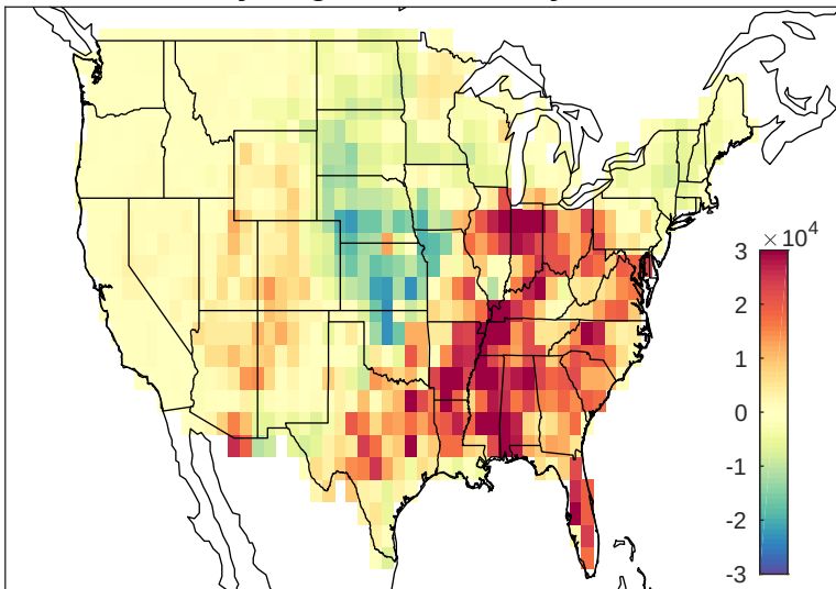
May-Aug NLDN anomaly 2003
