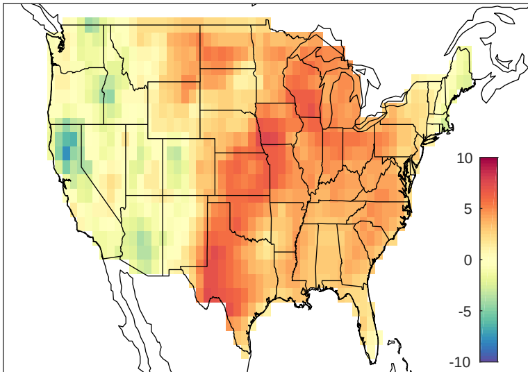
May-Aug 2-m dew-point temperature anomaly 2011
