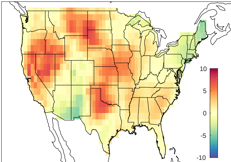
May-Aug 2-m dew-point temperature anomaly 2006
