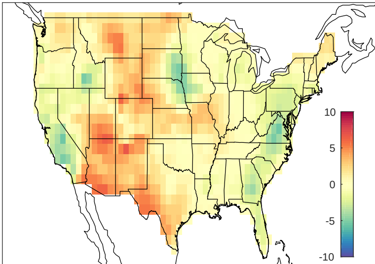
May-Aug 2-m dew-point temperature anomaly 2005
