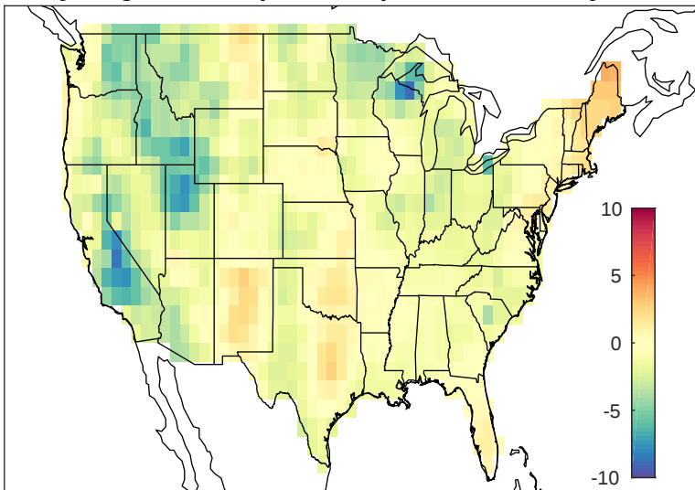
May-Aug 2-m dew-point temperature anomaly 2003
