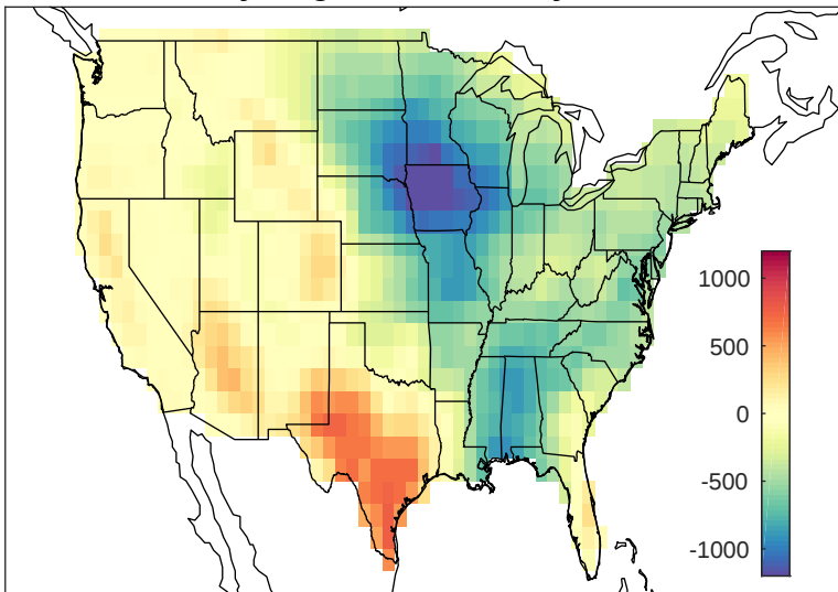
May-Aug CAPE anomaly 2016
