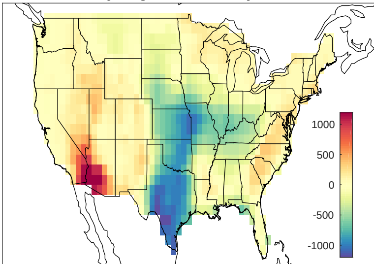
May-Aug CAPE anomaly 2008
