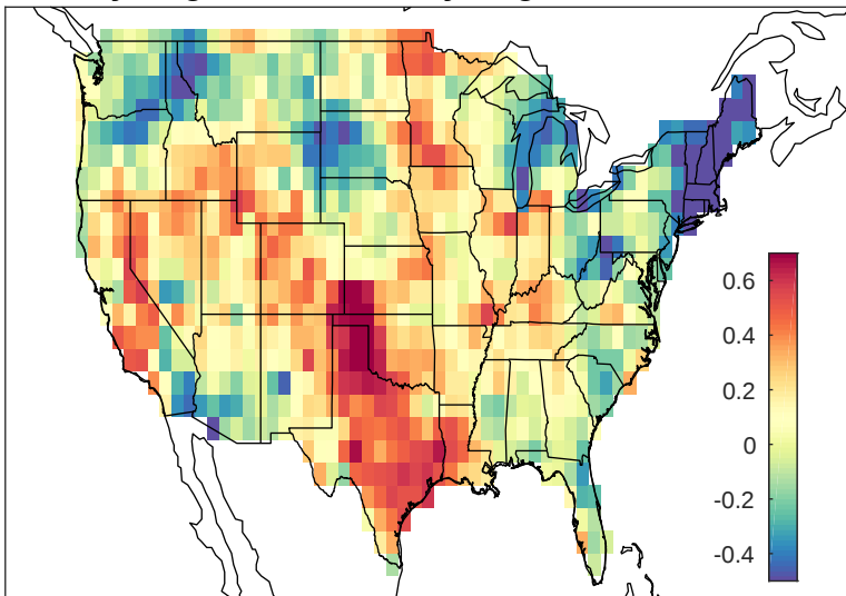
May-Aug cPRCP and May-Aug PDO 2003-2016
