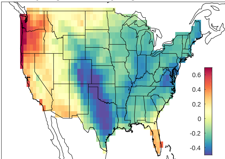
May-Aug t2m and May-Aug PDO 1996-2016
