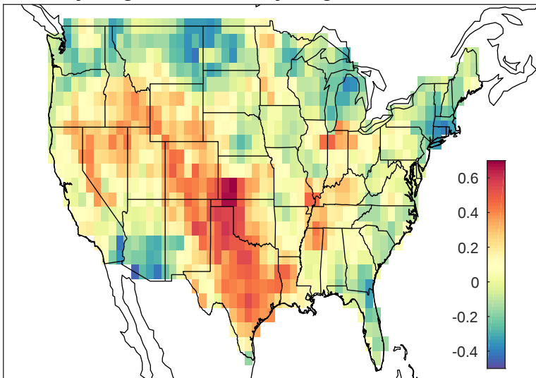
May-Aug PRCP and May-Aug PDO 1996-2016
