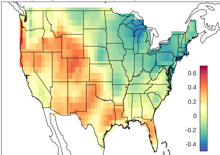
May-Aug CAPE and May-Aug PDO 1979-2016
