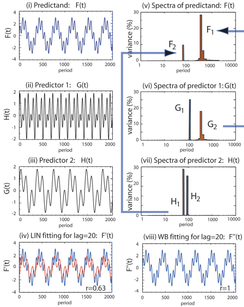
FIG. A1. Example of the WB method. (i) A simple periodic predictand F(t) is chosen with two periodic predictors (ii) G(t) and (iii) H(t) . Using a linear regression technique (e.g., LIN) to forecast 20 lags produces (iv) the function F'(t) . The correlation between F(t) and F'(t) is 0.63. However, if the spectra of the (v) predictand is noted and a spectral (or wavelet) banding applied in which (vi), (vii) the predictors are also banded, only part of the predictor functions will be used to predict. Predictor components T_1(t) and H_1(t) are discarded and G_2(t) is used to predict component F_2(t) and H_1(t) component F_1(t) (large blue arrows). The result for this simple case is (viii) a perfect forecast F''(t) .
