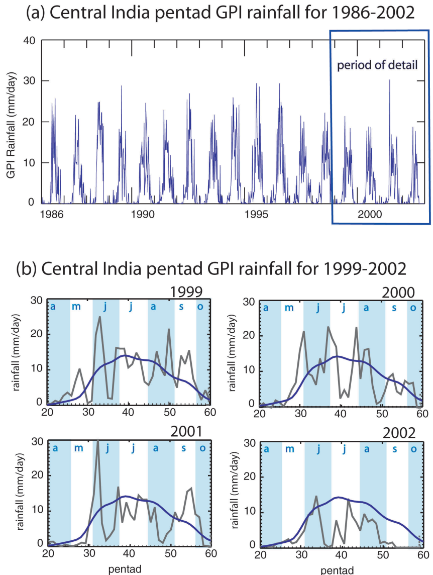
FIG. 2. (a) Satellite-derived GPI averaged over the central India region (see Fig. 1) for the period 1986–2002. A large annual cycle is modulated by a relatively small interannual variability. Within each summer season there are large variations of rainfall on time scales of 20–40 days. (b) Details of precipitation for the period 1999–2002 [box in (a)] plotted as average rain rate per pentad. Each year exhibits peaks (“active” monsoon periods) and valleys (“breaks” in the monsoon) of rainfall rate. The smoothness of the long-term averaged annual cycle of precipitation (blue curve) suggests that there is no preferred timing for intraseasonal variability and that it occurs randomly throughout the summer. Light-blue and white background bands indicate months (“a” April, “m” May, etc.). Data from Joyce and Arkin (1997).
