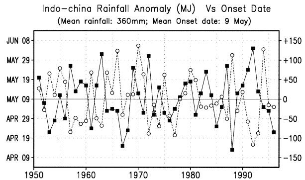
FIG. 13. The monsoon onset date and interannual anomaly of rainfall over Indochina during May–Jun in units of mm.
