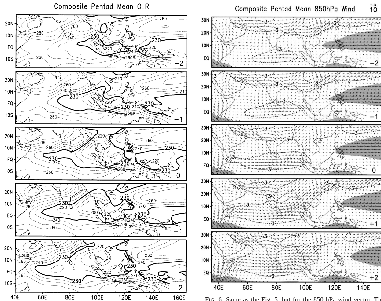
FIG. 5. Pentad mean evolution of the composite OLR with centering the onset dates. Here "0" denotes onset pentad and "-" and "+" refer to prior to and after onset pentad, respectively. See text for detail about the definition of the onset pentad. The interval of the contour is 10 \text{ W m}^{-2} with the 230 \text{ W m}^{-2} contour denoted by the thick solid line. To minimize the seasonal background differences in the extreme early and late onset years, the years of onset dates earlier than 25 Apr or later than 25 May are excluded from the composite.
