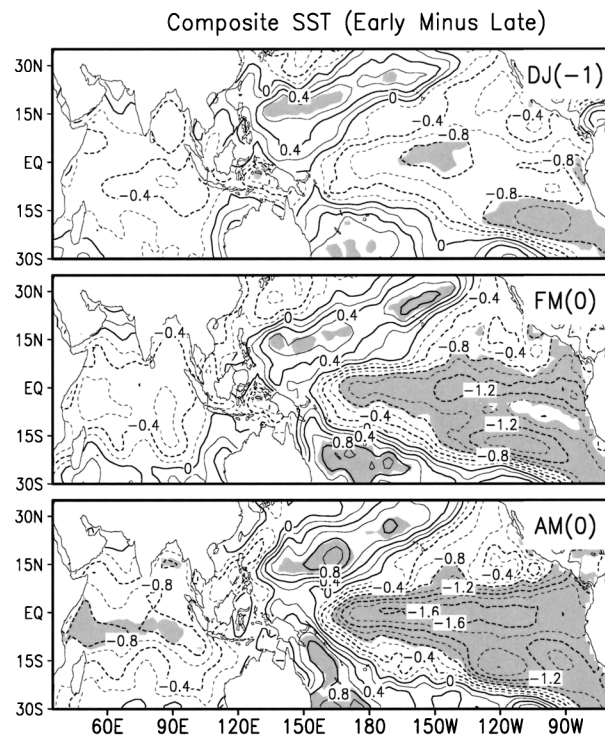
FIG. 14. The bimonthly early-minus-late composite of SST from preceding winter to spring. The interval is 0.1^{\circ}\text{C} . The “0” denotes the year of the reference monsoon year. Shading indicates that the t test passes the 5% significance level.
