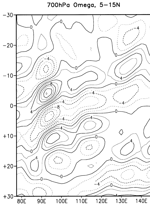
FIG. 12. The longitude–time cross section of the composite filtered omega at 700 hPa for the phase-locking years along 5°–15°N in units of 0.001 \text{ Pa s}^{-1} . The interval is 0.002 \text{ (Pa s}^{-1}\text{)} .
