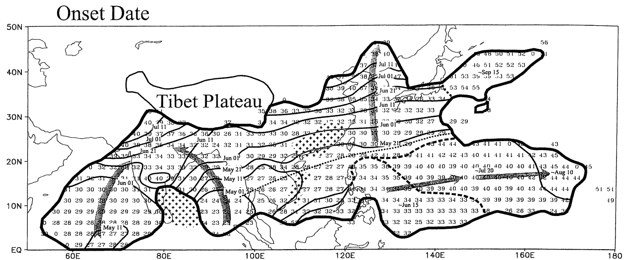
FIG. 1. Mean onset date of the Asian summer monsoon adopted from Wang and LinHo (2002). The number is the onset (Julian) pentad. The thick dashed lines denote discontinuities (merger of three or more contours). The arrows point to the directions of rain-belt propagation. The thin dashed line divides subtropical monsoon and oceanic monsoon regions. The Tibetan Plateau is outlined by the 3000-m contour.
