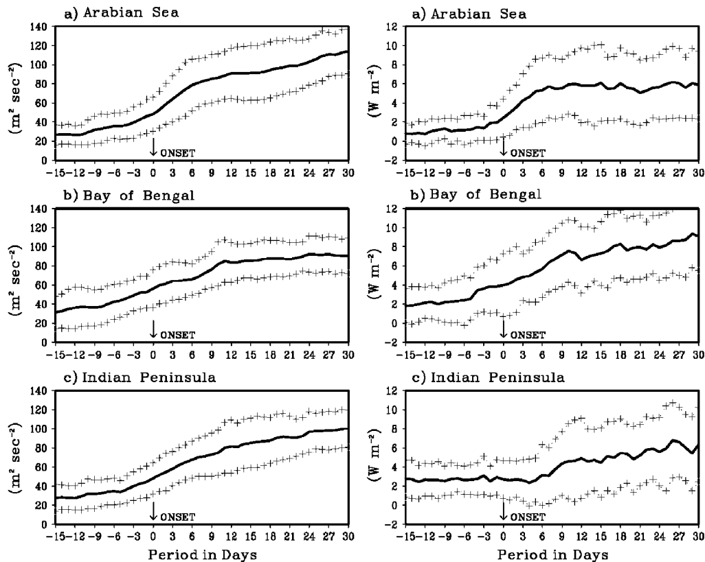
Figure 10. Evolution of kinetic energy at 850 hPa ( \text{m}^2 \text{s}^{-2} ) (left panels) and volume-integrated generation of kinetic energy ( \text{W m}^{-2} ) (right panels) during the onset phase over Kerala for (a) Arabian Sea, (b) Bay of Bengal, (c) Indian Peninsula (the + symbols represents the upper and lower bounds of standard deviation from the mean value)
