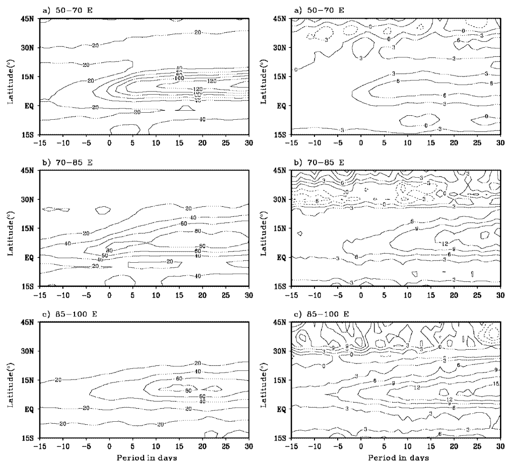
Figure 9. Time-latitude variations of kinetic energy at 850 hPa ( \text{m}^2 \text{s}^{-2} ) (left panels) vertically integrated generation of kinetic energy ( \text{W m}^{-2} ) (right panels) for (a) Arabian Sea, (b) Indian Peninsula and (c) Bay of Bengal
