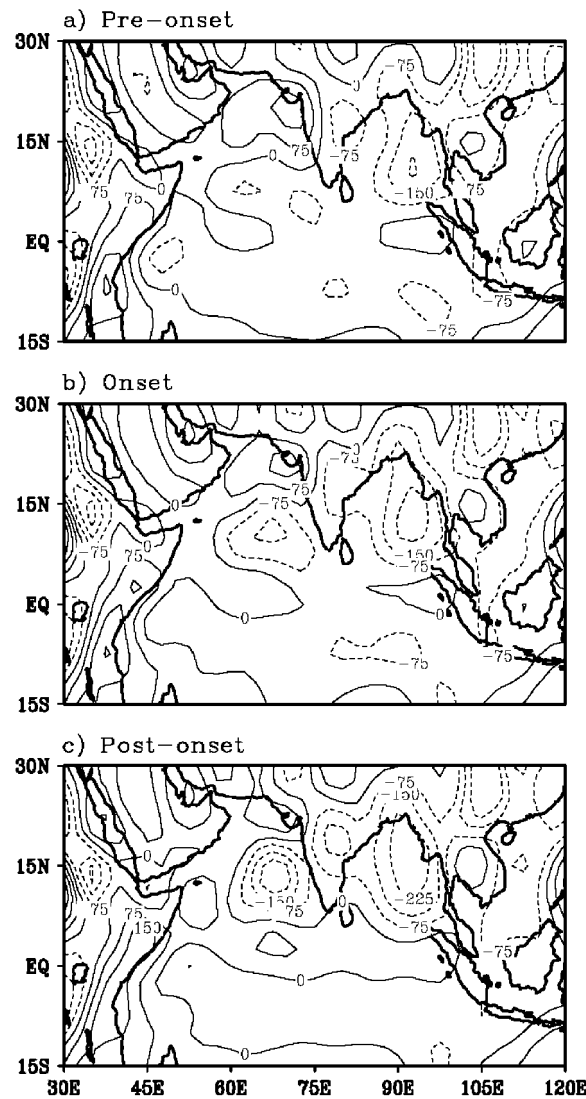
Figure 8. Geographical distribution of vertically integrated horizontal divergence flux of moisture ( \text{W m}^{-1} ): (a) pre-onset, (b) onset, (c) post-onset
