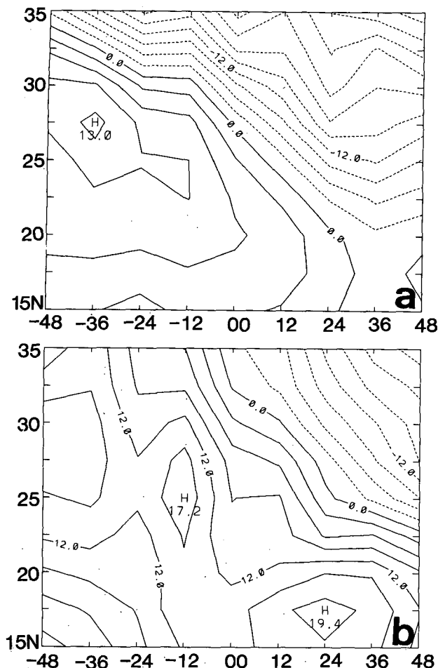
FIG. 5. Time-latitude sections of the composite geopotential height anomaly (departure from the monthly mean) averaged over 1000-, 850-, and 700-hPa and between 112.5° and 117.5°E for (a) the monsoon onsets and (b) the June surges. The unit is geopotential meter (gpm), and negative contours are indicated by dashed lines.
