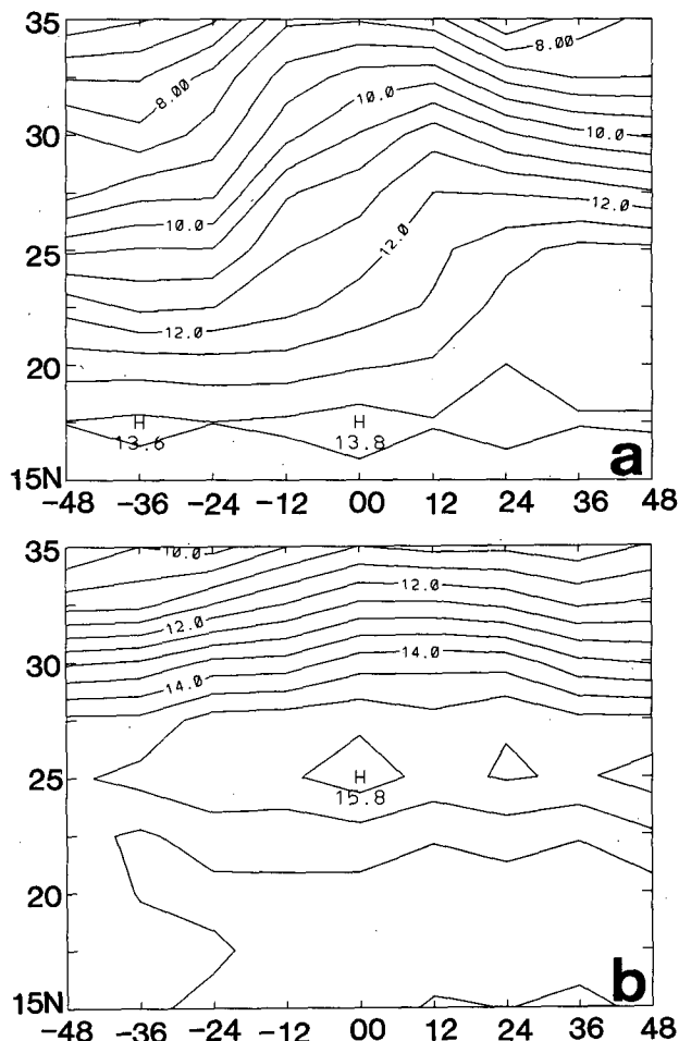
FIG. 6. As in Fig. 5 except for mixing ratio ( \text{g kg}^{-1} ).
