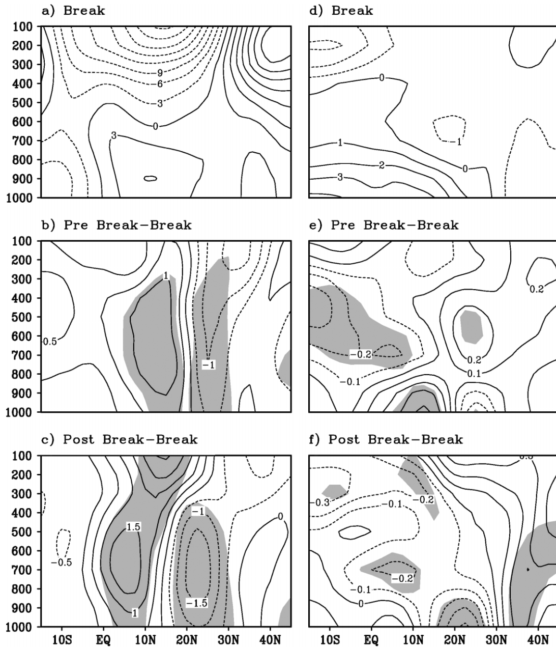
Figure 3. Sectorial mean ( 30\text{--}120^\circ\text{E} ) vertical cross-sections of zonal wind ( \text{m s}^{-1} ) for (a) break (b) pre-break-break, (c) post-break-break. (d), (e) and (f) Same as (a), (b) and (c) respectively, but for meridional wind ( \text{m s}^{-1} ) with confidence limits above 95% (shaded)
