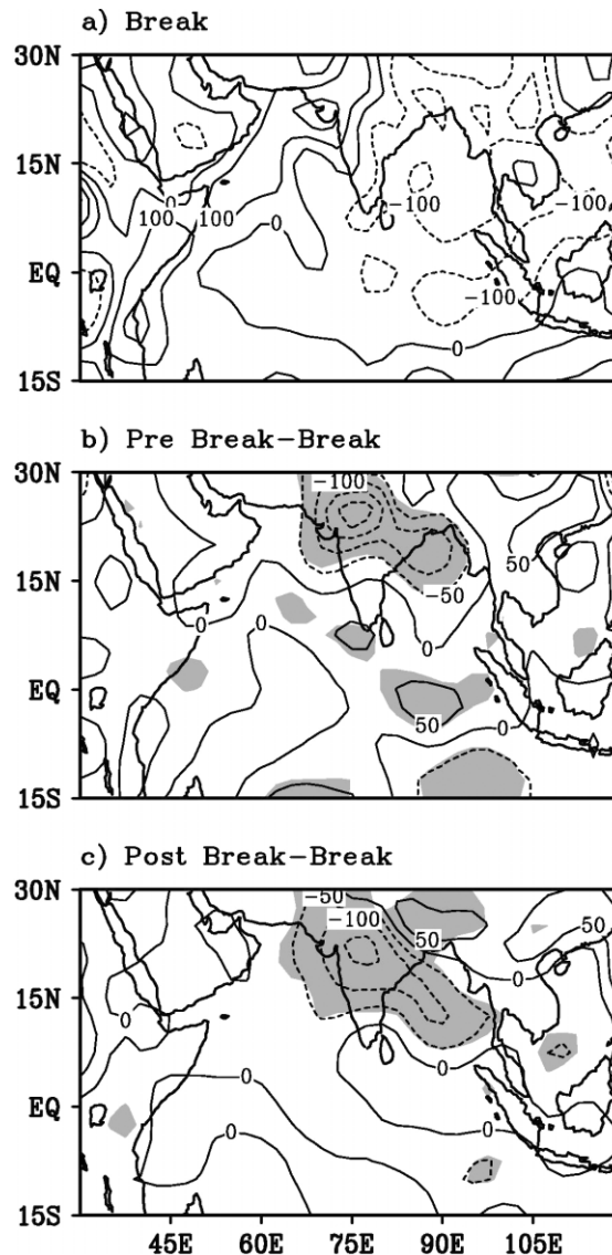
Figure 11. Geographical distributions of vertically integrated horizontal flux of moisture ( \text{W m}^{-2} ) for (a) break, (b) pre-break–break, (c) post-break–break with confidence limits above 95% (shaded)
