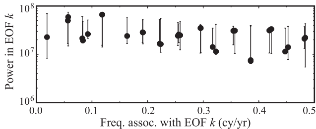
Figure 1. SSA eigenvalue spectrum and 90% red-noise confidence interval, computed using a Monte Carlo method with 1000 realizations.
