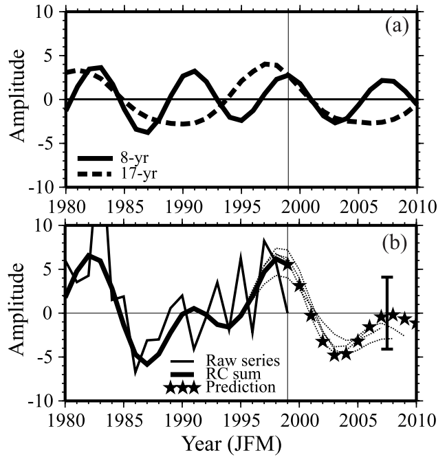
Figure 5. The RCs 1–2 and 3–4 computed over 1904–99 with M = 30 , plotted 1980–99, together with their predictions (5 LP coefficients) made from 1999. (a) Individual RC sums and predictions, (b) combined sum (thick solid line) and prediction (stars), and raw JFM flow anomalies (thin line). The thin dotted curves in panel (b) show four predictions starting in 1995, 1996, 1997 and 1998 respectively. Units: 10^3 \text{ m}^3\text{s}^{-1} .
