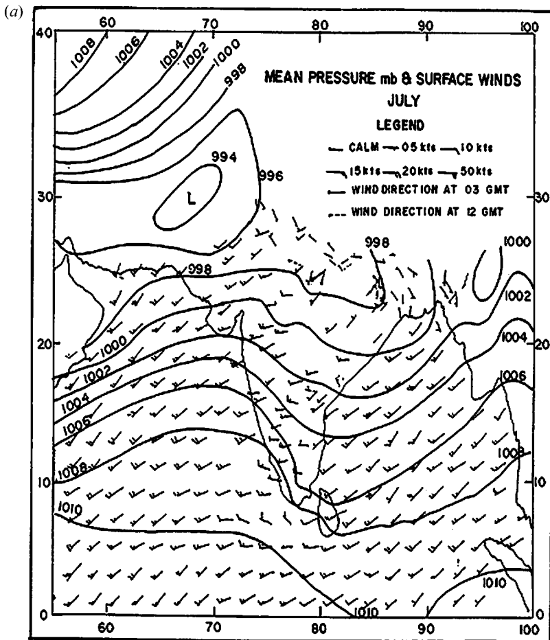
Figure 1 Mean surface winds and pressure for July (a) and January (b) (after Rao 1976).
