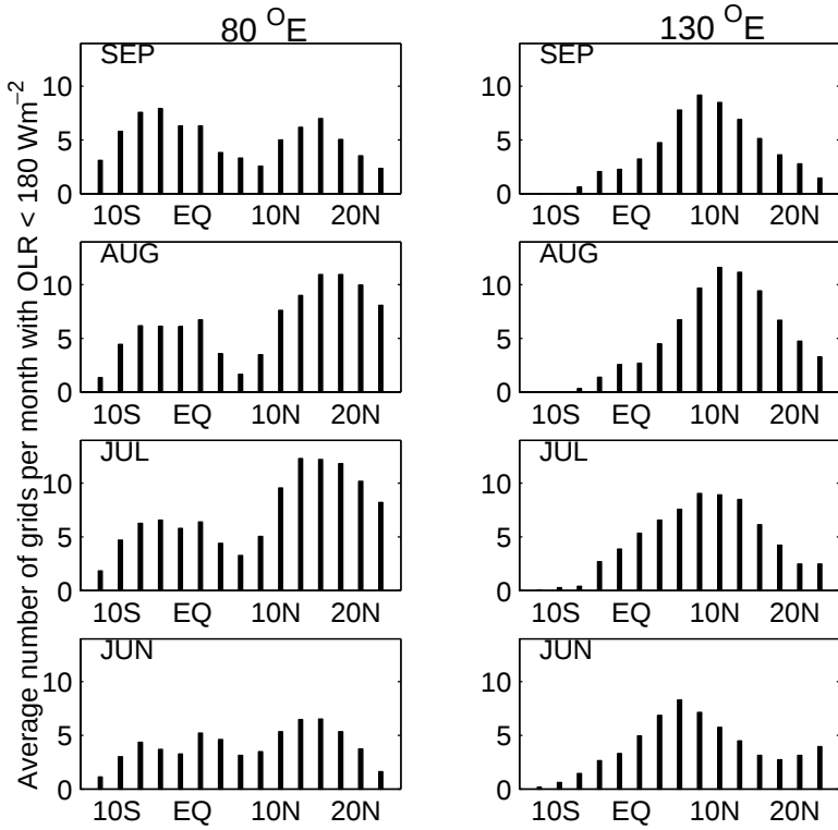
Figure 8 Variation of the occurrence of days in a month with OLR less than 180 \text{ Wm}^{-2} , with latitude at 80^\circ\text{E} (central longitude of the Indian region) and 130^\circ\text{E} over the western Pacific for June to September.
