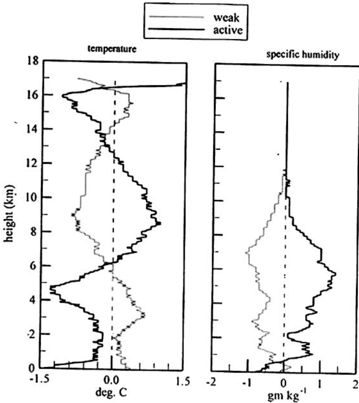
Figure 18 Composite vertical profiles of temperature and specific humidity anomalies for active and weak spells over the Bay of Bengal during BOBMEX (after Bhat et al. 2002).
