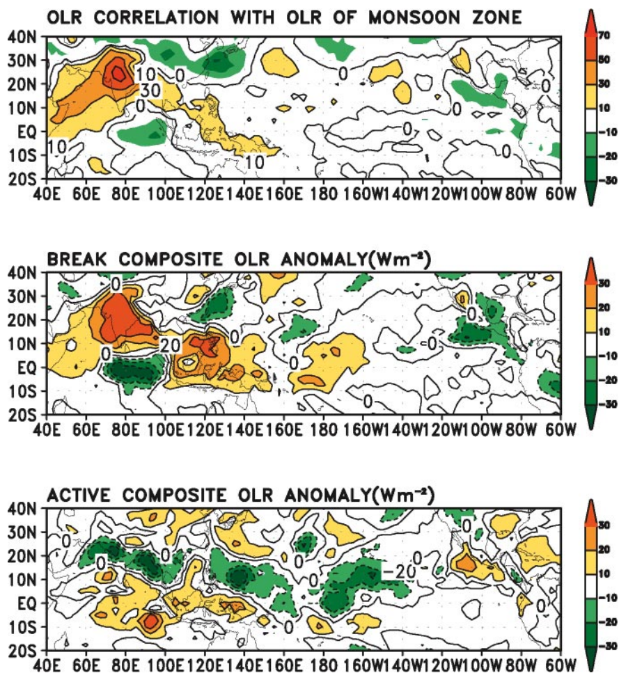
Figure 11 (a) Correlation of three-day running mean OLR with respect to that of the OLR of the monsoon zone (Figure 4a) for July–August. (b) Break composite OLR anomaly patterns (after Gadgil & Joseph 2003). (c) Active composite patterns of OLR and OLR anomaly patterns (after Gadgil & Joseph 2003).
