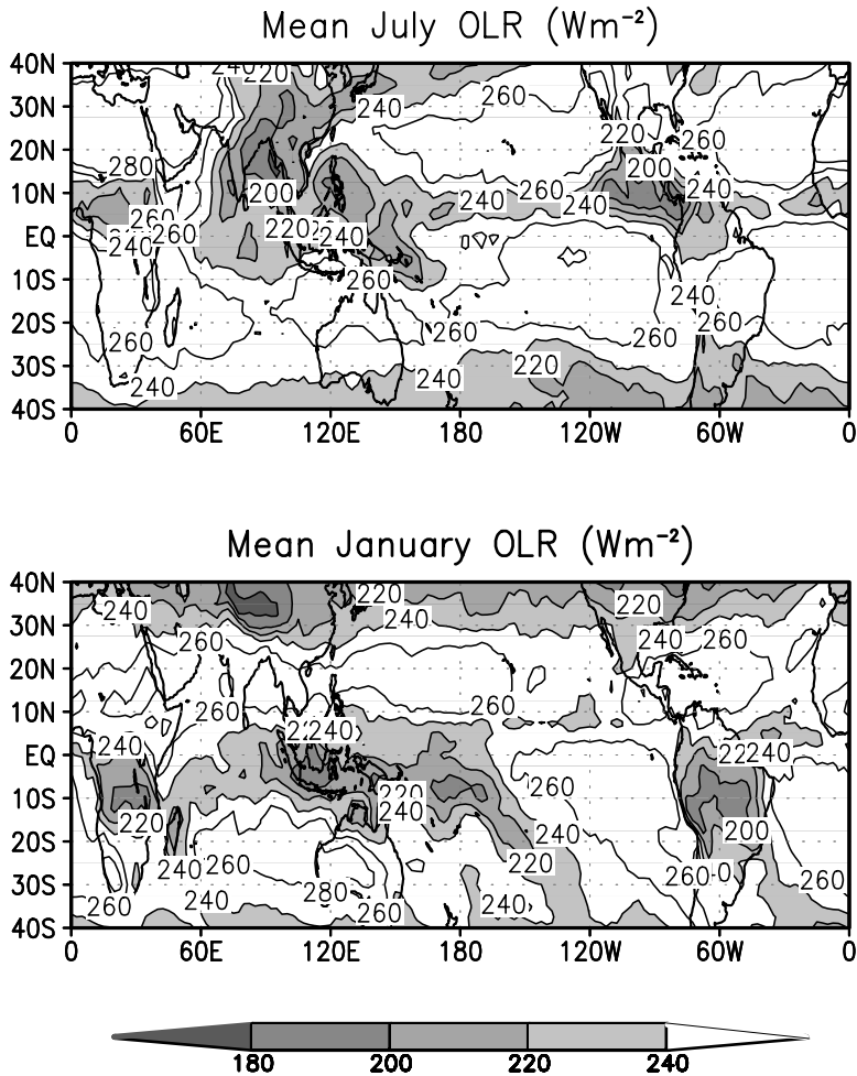
Figure 7 Mean OLR ( \text{wm}^{-2} ) for January and July from data of Walisser & Zhou (1997).
