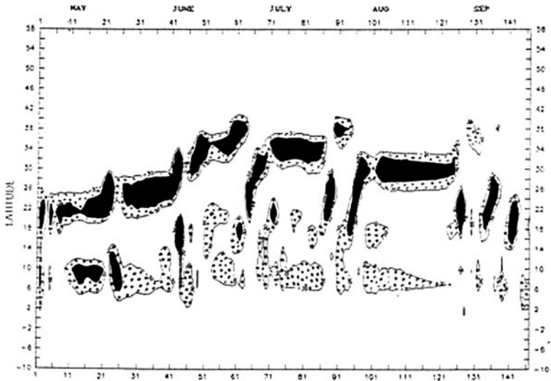
Figure 12 Simulation of intraseasonal variation of TCZ with a simple axisymmetric model by Nanjundiah et al. (1992).
