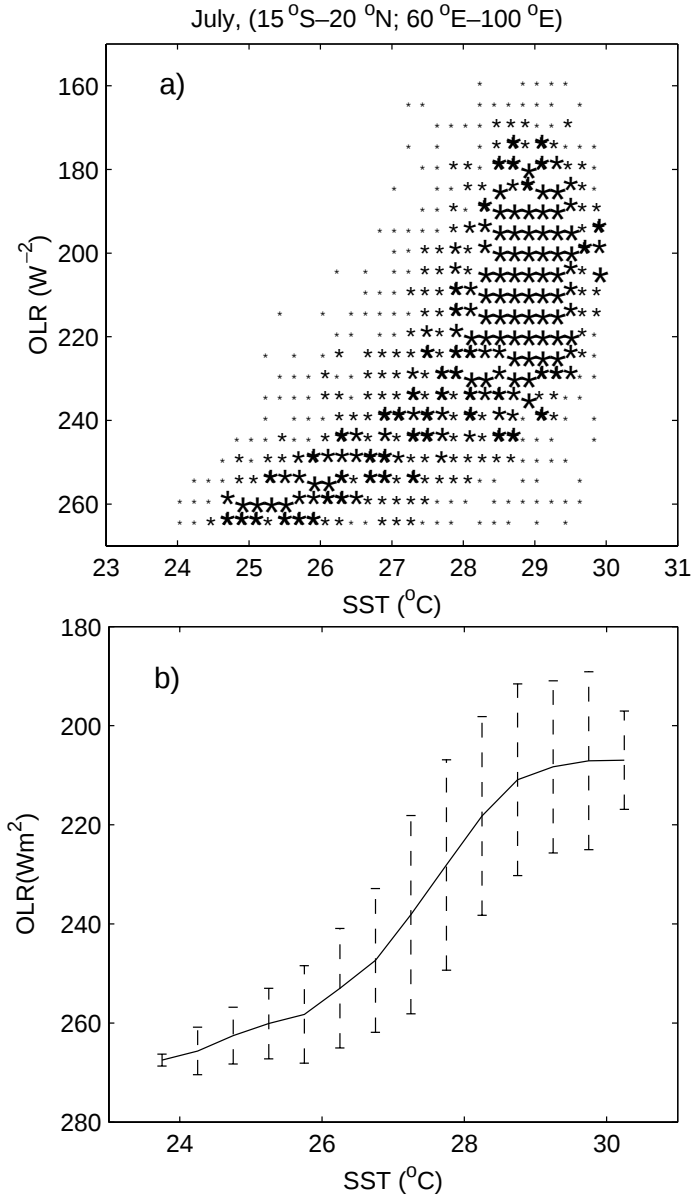
Figure 14 For July (1982–1998) over the Indian Ocean ( 15^{\circ}\text{S} – 20^{\circ}\text{N} , 60^{\circ}\text{E} – 100^{\circ}\text{E} ). (a) Variation of OLR and SST. (b) Variation of the mean and standard deviation of OLR with SST.
