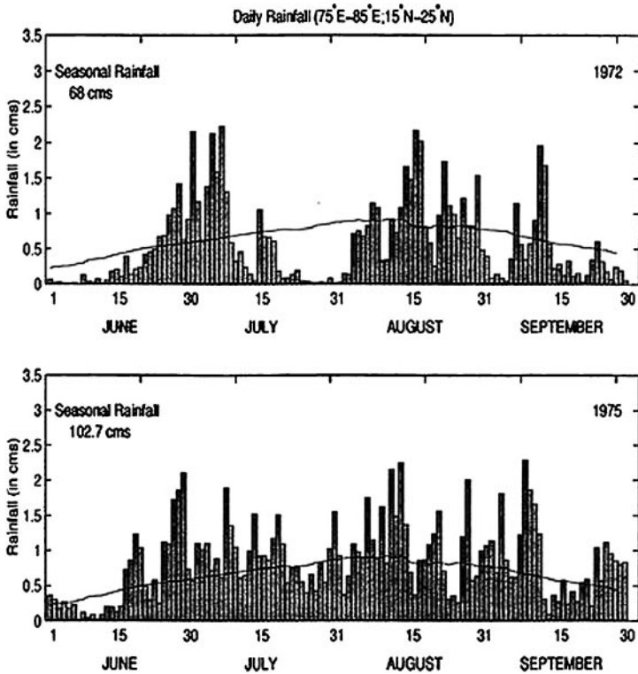
Figure 5 Variation of daily rainfall over central India during 1972 and 1975.
