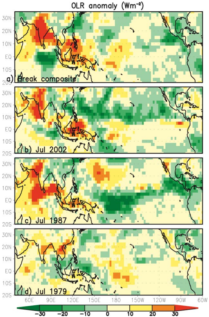
Figure 13 OLR anomaly patterns for (a) the break composite, (b) July 2002, (c) July 1987, and (d) July 1979.
