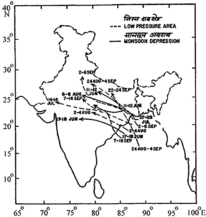
Figure 6 Paths of low pressure systems during the summer monsoon season of 1999.
