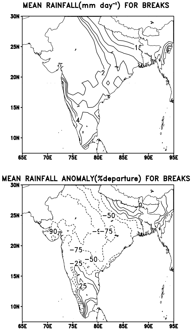
Figure 10 Break composite patterns of rainfall and rainfall anomaly (after Gadgil & Joseph 2003).
