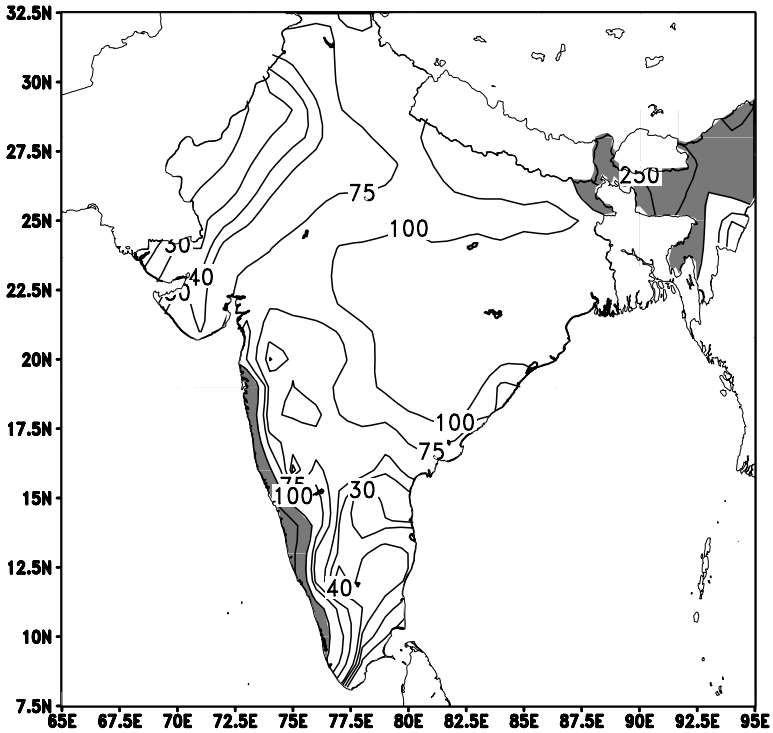
Figure 2 Mean June–September rainfall over the Indian region south of 30^{\circ} N.
