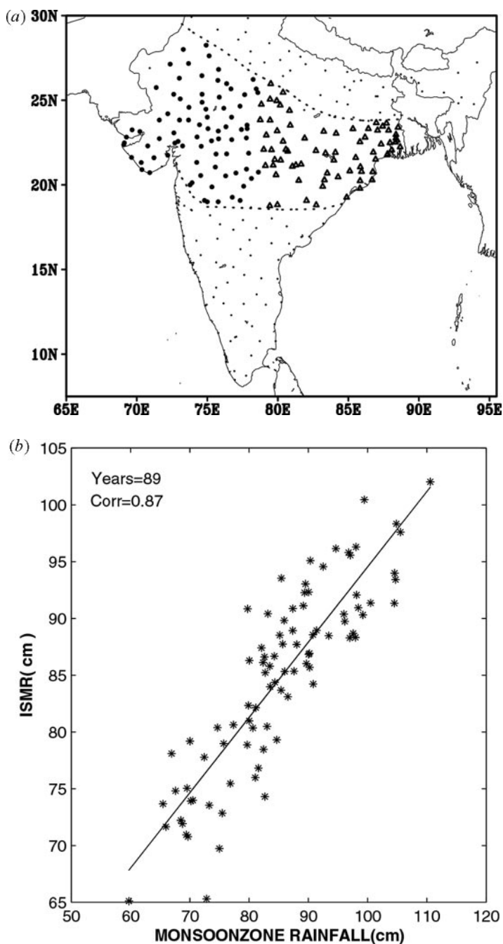
Figure 4 (a) The Indian monsoon zone (limits indicated by dashed lines ) and the network of stations. Stations in the western and eastern parts of the monsoon zone indicated by circles and triangles. (b) ISMR versus June–September rainfall over the monsoon zone; sample size (89 years) and correlation (0.87) are indicated.
