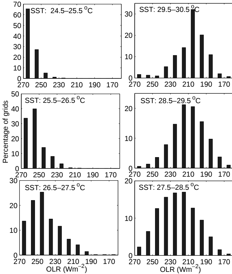
Figure 15 For July (1982–1998) over the Indian Ocean, percentage of grids in different OLR ranges for specified SST ranges.
