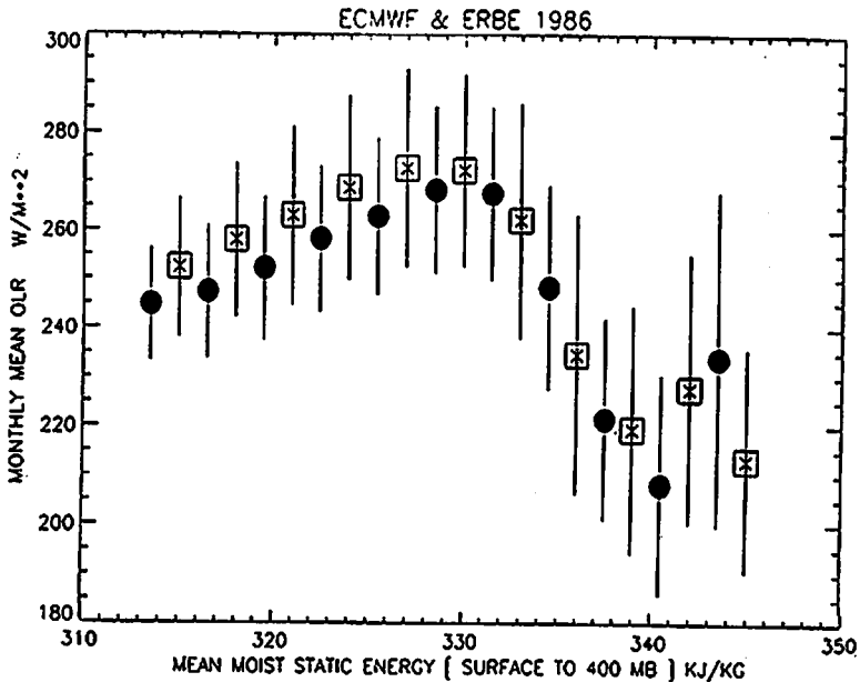
Figure 17 OLR versus lower tropospheric moist static energy for grids over land ( squares ) and ocean ( solid circles ), after Srinivasan & Smith (1996).
