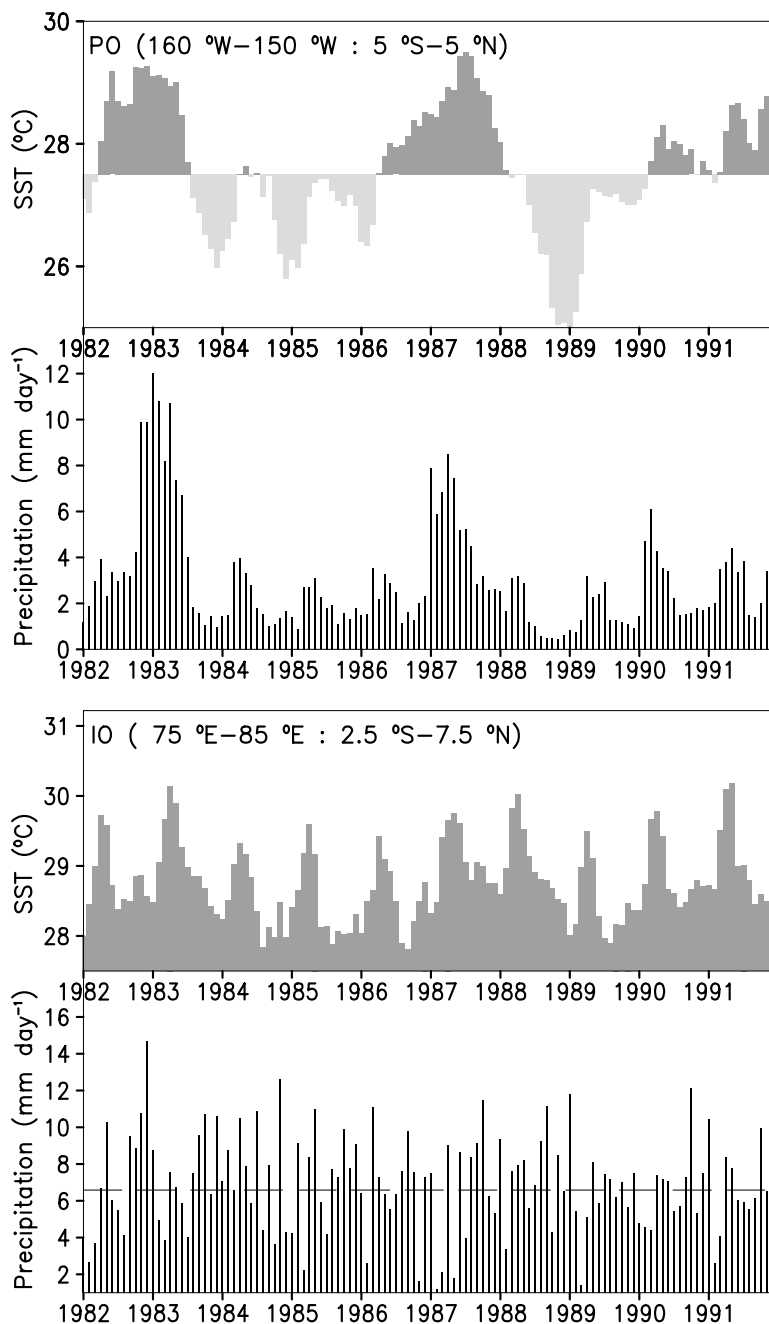
Figure 16 Variation of monthly SST and MSU precipitation over parts of the Pacific and Indian Oceans.
