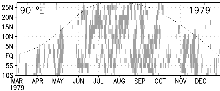
Figure 9 Variation of the grids with OLR less than 200 and 180 \text{ Wm}^{-2} at 90^\circ\text{E} during March–December 1979. The seasonal envelope is also indicated.
