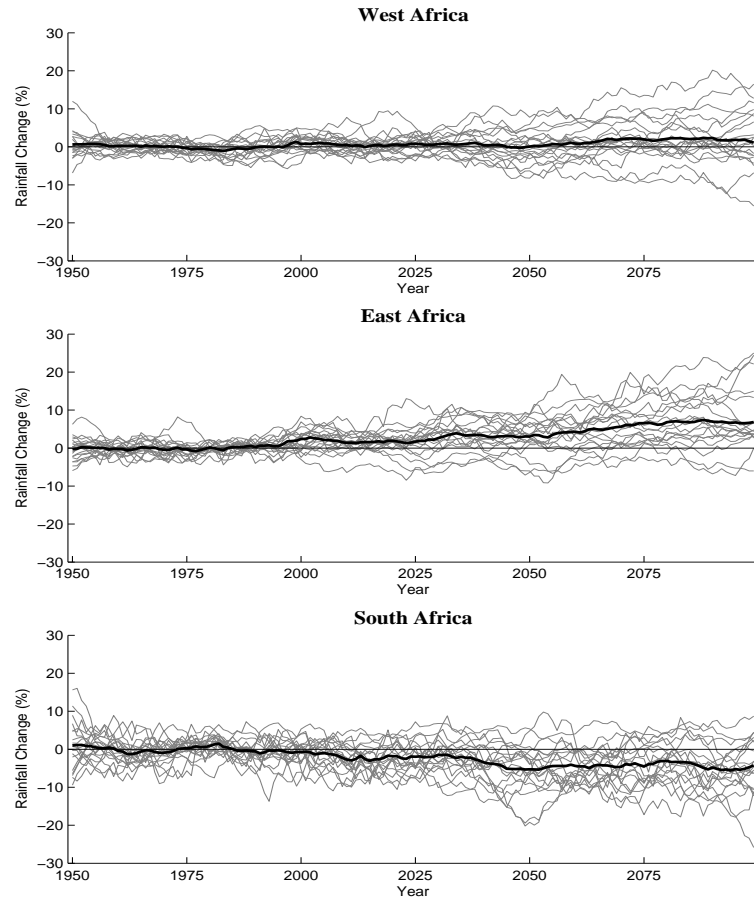
Figure 6. Regional averages of precipitation in the IPCC 4AR model simulations; 20th century simulations from 1950 to 2000, and A1B scenario simulations from 2000 to 2100. Regions are defined as in figure 2. Each grey line represents one model, and the thicker black line is the multi-model mean.
