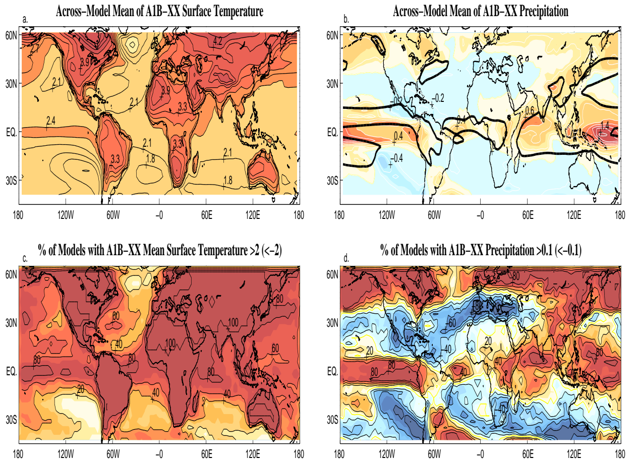
Figure 5. As for figure 4, but for the A1B-XX difference. In the top panels, the shading (contour) interval is 0.6^{\circ}\text{C} ( 0.3^{\circ}\text{C} ) for temperature and 0.15 \text{ mm day}^{-1} ( 0.2 \text{ mm day}^{-1} ) for rainfall. In the bottom left panel the threshold is 2^{\circ}\text{C} , while in the bottom right panel it is 0.1 \text{ mm day}^{-1} .
