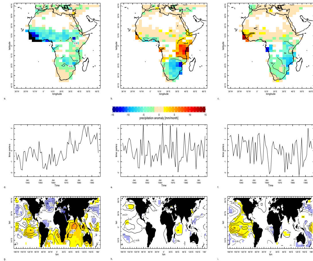
Figure 3. The three leading patterns of a Principal Component Analysis performed on annual mean (July-June) precipitation over Africa during 1930-1995. a, b, c: The spatial patterns, obtained by linear regression of the time series in d,e,f onto precipitation - anomalies are in color, in mm/month, while the contours delimit regions where regression is statistically significant at the 5% level. d, e, f: The associated time series (in units of standard deviation). Note that the upward trend in (d) indicates increasingly stronger values of the negative anomalies in the pattern in (a), i.e. a drying trend. g, h, i: Regression patterns of the time series in d,e,f with sea surface temperature (Kaplan et al. 1998). Anomalies are in contour, spaced every 0.05^{\circ}\text{C} , and dashed in the case of negative values; the presence of color represents their statistical significance at a level of 5% or higher.
