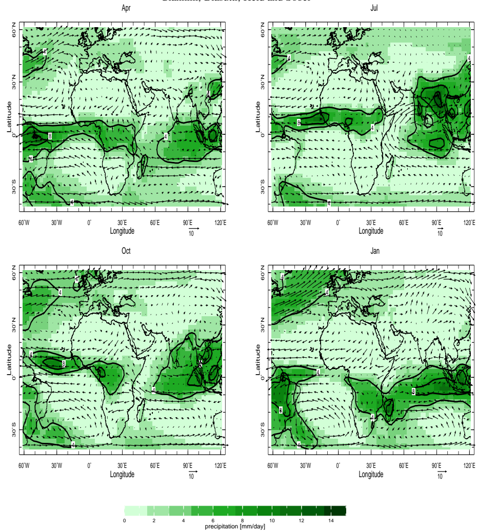
Figure 1. Climatologies of precipitation and near-surface winds for a domain centered on tropical Africa. Precipitation was produced by the Global Precipitation Climatology Project (Huffman et al. 1997) combining satellite estimates and rain-gauge measurements (contours are drawn every 4 mm/day). Winds at the 850hPa pressure level - approximately 3000m above sea level - are from the NCEP-NCAR Reanalysis Project (Kalnay et al. 1996). Panels are for April, July, October and January averages over 1979-2004.
