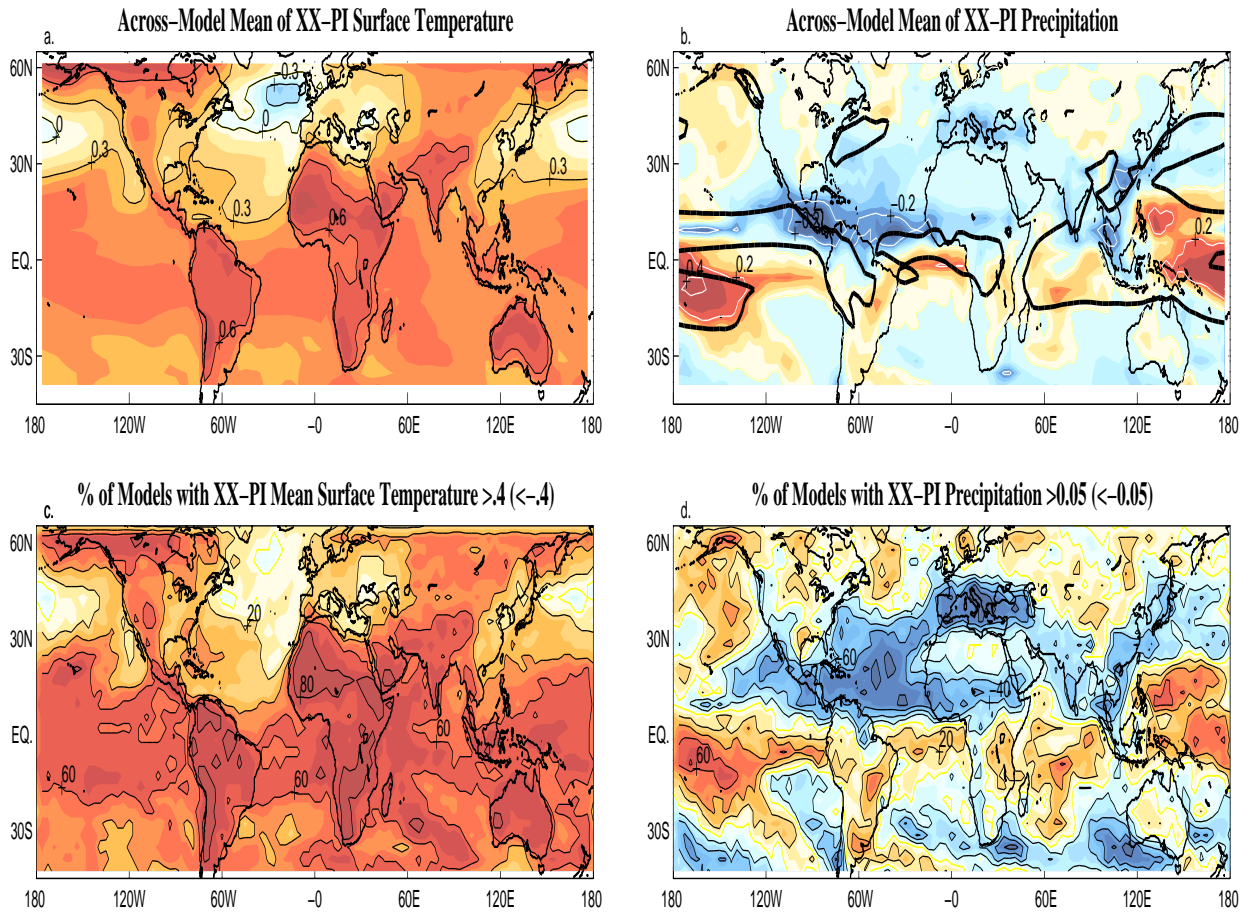
Figure 4. difference (XX-PI) between late 20th century (1975-1999) climate in the XX simulations and pre-industrial climate, as estimated from a 25-year mean from the PI simulations. The left panels refer to annual mean surface temperature, the right panels to annual mean precipitation. Warm colors indicate positive and cool colors negative anomalies. The top panels are the mean across all 19 models (the shading interval is 0.1^{\circ}\text{C} for temperature and 0.03\text{mm day}^{-1} for precipitation), the solid black line in the right panel is the 4\text{mm day}^{-1} contour in the XX simulations and indicates the location of mean maximum rainfall. The bottom panels are a measure of inter-model agreement: a value of 1 (-1) was assigned at every gridpoint and for every model if the XX-PI difference was positive (negative) and larger than a threshold ( 0.4^{\circ}\text{C} or 0.05\text{mm day}^{-1} ) value; the panels show the sum over all models as percentages (shading interval is every 10%, contour interval is every 20%).
