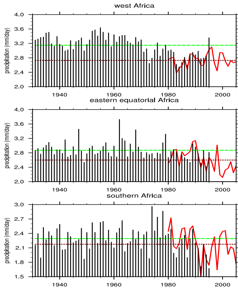
Figure 2. Regional averages of annual mean (July-June) precipitation over 1930-2005; the three regions are western ( 0^{\circ}\text{N} to 20^{\circ}\text{N} , 20^{\circ}\text{W} to 20^{\circ}\text{E} ), eastern equatorial ( 10^{\circ}\text{S} to 10^{\circ}\text{N} , 20^{\circ}\text{E} to 50^{\circ}\text{E} ), and southern Africa ( 25^{\circ}\text{S} to 10^{\circ}\text{S} , 20^{\circ}\text{E} to 40^{\circ}\text{E} ). CRU data is depicted in black bars, GPCP in the solid red line. The CRU climatology over 1930-1995 is depicted in the green horizontal line, that of GPCP, over 1979-2005, is depicted in the brown horizontal line.
