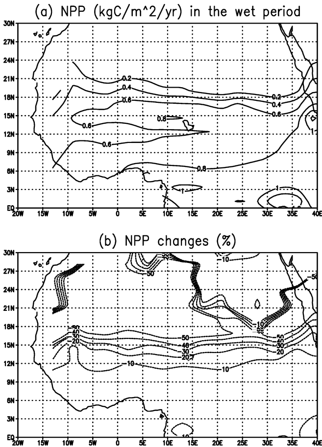
Fig. 6 a Net primary productivity (in \text{kgC/m}^2/\text{year} ) averaged during the wet 1950s, simulated by the experiment Veg_Dynamic at R30 resolution; b decrease of net primary productivity from the 1950s to the dry period after 1970
