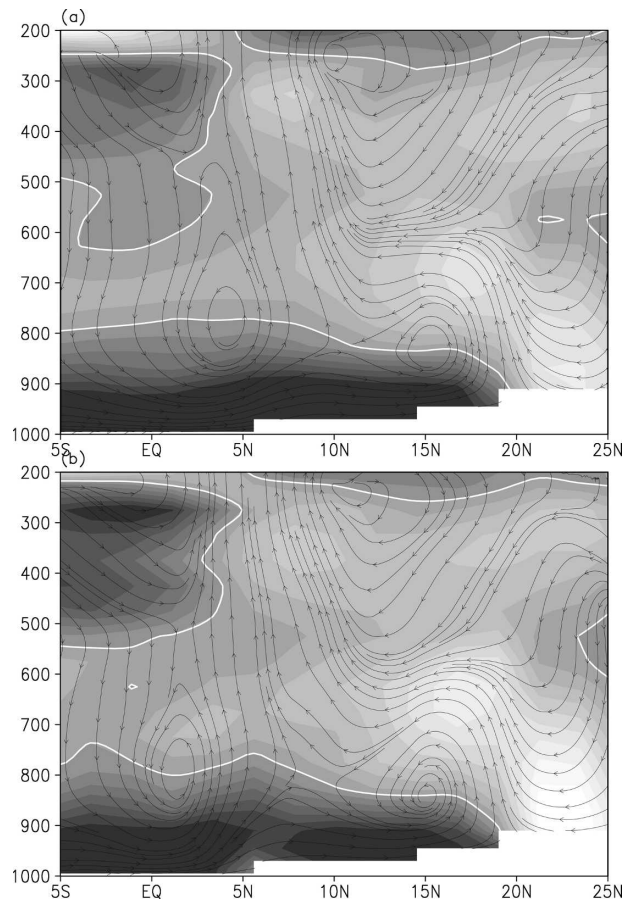
FIG. 4. (a) Latitude–height cross section of streamlines ( v, w \times 10^{-2} ) along 5°E longitude from VC02's regional climate model simulations averaged over JJAS. Shading indicates meridional wind speeds with 1 \text{ m s}^{-1} intervals. The thick white line indicates the zero meridional velocity contour, and darker shades mark positive (northward) velocity. (b) Same as in (a), but when warming is imposed in the Gulf of Guinea in the model.
