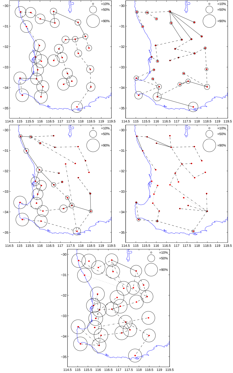
Figure 11: Graphical interpretation of the hidden states for a 5-state HMM-CL trained on South-western Australia data. Circle radii indicate the precipitation probability for each station given the state. Lines between the stations indicate the edges in the graph while different types of lines indicate the strength of mutual information of the edges.
