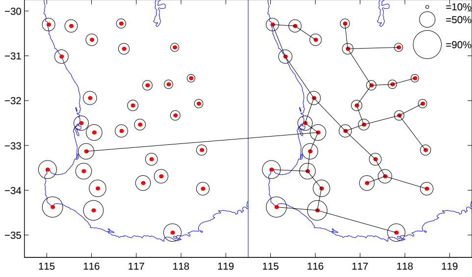
Figure 12: Graphical interpretation of the CCLF trained on Southwestern Australia data. Circle radii indicate the precipitation probability for each station. Lines between the stations indicate the edges in the graph while different types of lines indicate the strength of mutual information of the edges. The left side of the plot corresponds to observations \mathbf{R}_{t-1} while the right side to \mathbf{R}_t .
