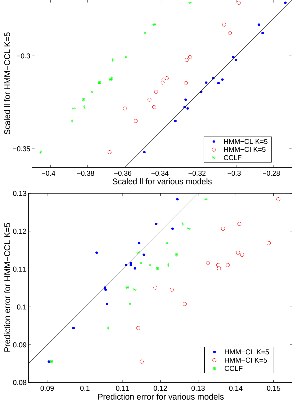
Figure 9: Southwestern Australia data: scatterplots of scaled log-likelihoods (top) and average prediction error (bottom) obtained by leave-one-winter-out cross-validation. The line corresponds to y = x . The independent chains model is not shown since it is beyond the range of the plot (average ll = -0.6034 , average error = 0.291).
