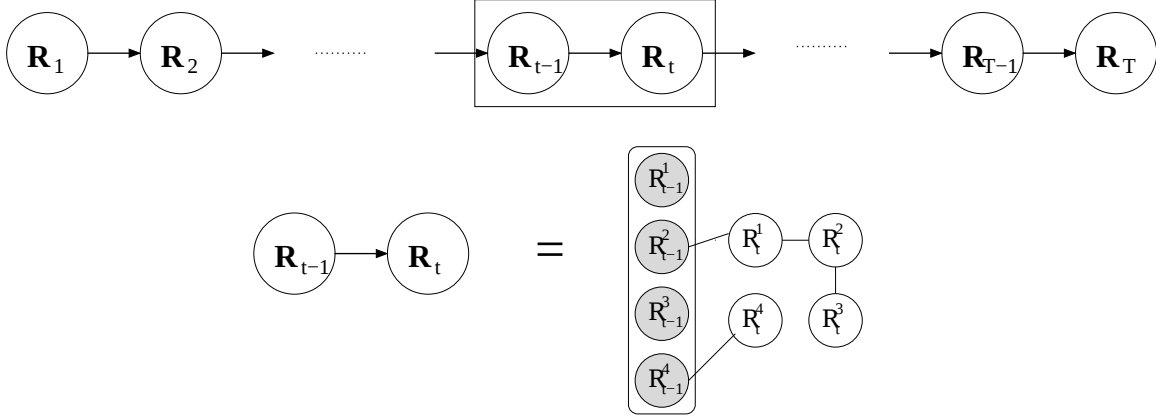
Figure 4: Graphical model for a hypothetical CCLF
