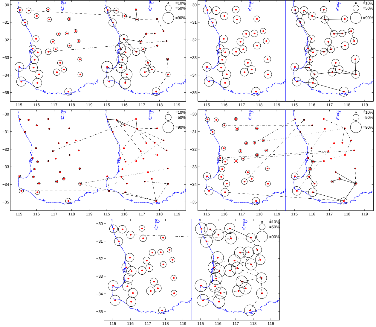
Figure 14: Graphical interpretation of the hidden states for a 5-state HMM-CCL trained on South-western Australia data. Circle radii indicate the precipitation probability for each station given the state. Lines between the stations indicate the edges in the graph while different types of lines indicate the strength of mutual information of the edges. The left side of the plot corresponds to observations \mathbf{R}_{t-1} while the right side to \mathbf{R}_t .
