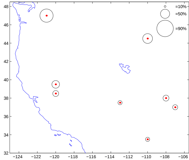
Figure 8: Stations in the Western U.S. region. Circle radii indicate marginal probabilities of rainfall ( > 0mm ) at each location.
