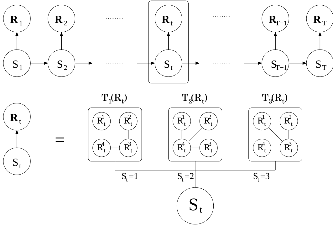
Figure 5: Graphical model interpretation of a hypothetical HMM-CL
