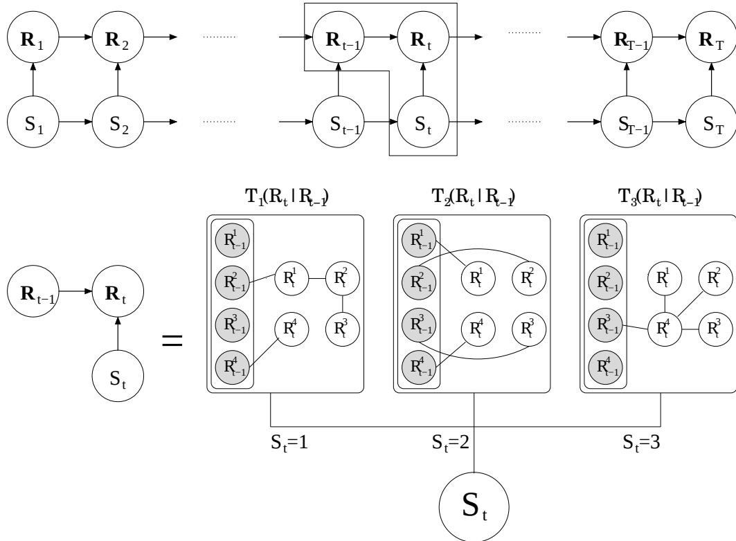
Figure 6: Graphical model interpretation of a hypothetical HMM-CCL
