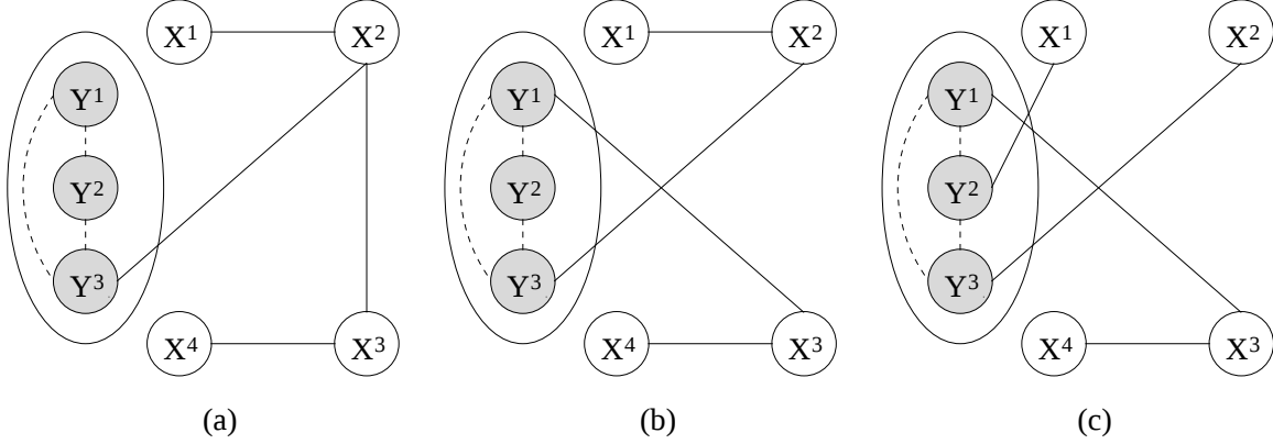
Figure 3: Conditional CL forest for a hypothetical distribution with (a) 1 component (b) 2 components (c) 3 components.
