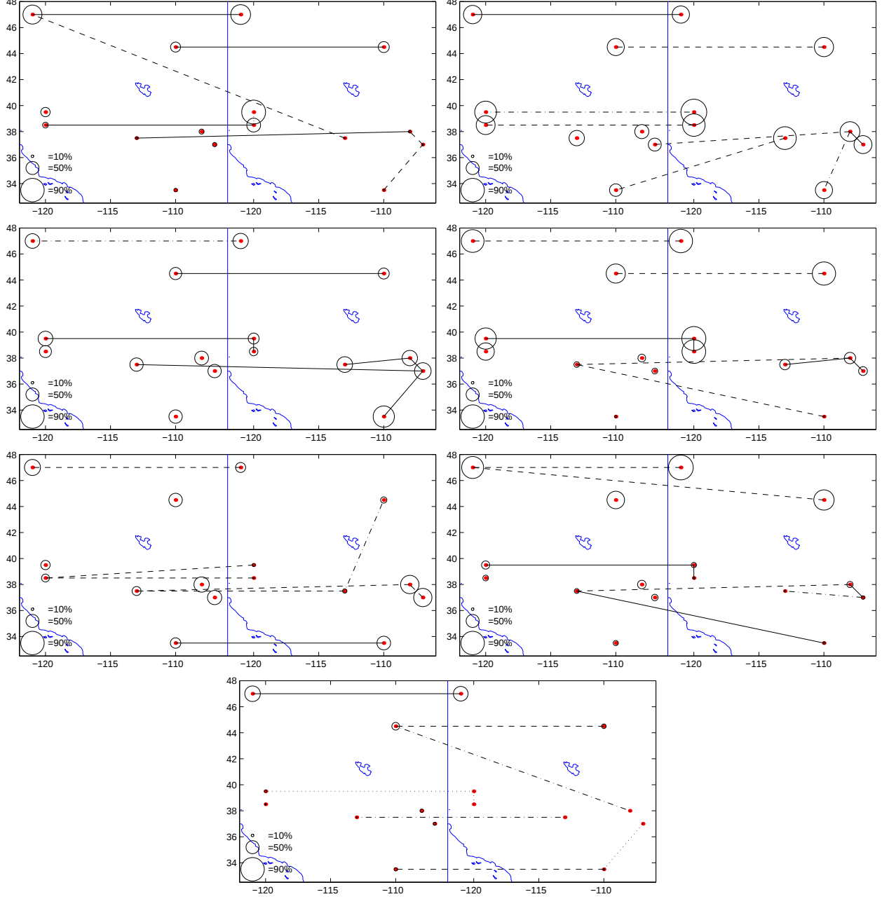
Figure 15: Graphical interpretation of the hidden states for a 7-state HMM-CCL trained on Western U.S. data. Circle radii indicate the precipitation probability for each station given the state. Lines between the stations indicate the edges in the graph while different types of lines indicate the strength of mutual information of the edges. The left side of the plot corresponds to observations \mathbf{R}_{t-1} while the right side to \mathbf{R}_t .
