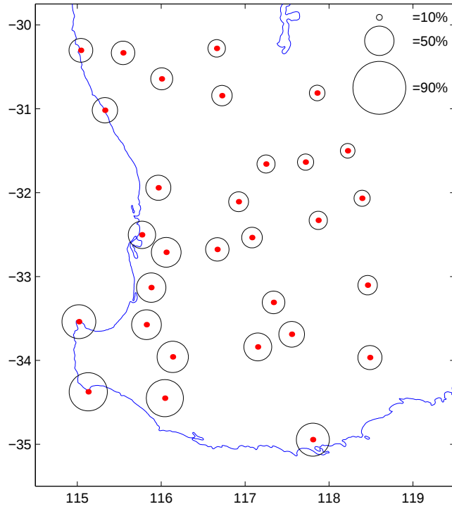
Figure 7: Stations in the Southwestern Australia region. Circle radii indicate marginal probabilities of rainfall ( > 0.3mm ) at each location.
