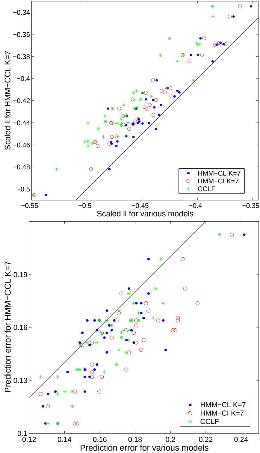
Figure 10: Western U.S. data: Scatterplots of scaled log-likelihoods (top) and average prediction error (bottom) obtained by leave-one-winter-out cross-validation. The line corresponds to y = x . The independent chains model is not shown since it is beyond the range of the plot (average l = -0.5204 , average error = 0.221).
