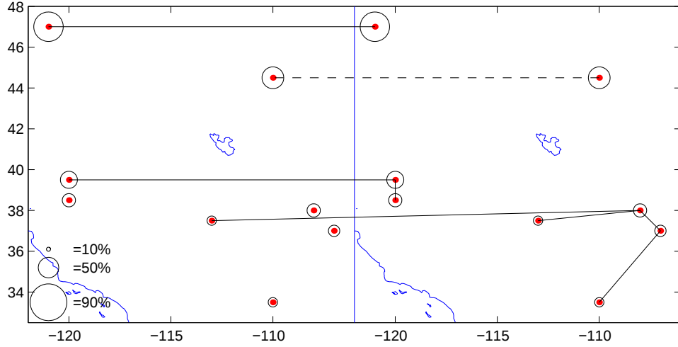
Figure 13: Graphical interpretation of the CCLF trained on Western U.S. data. Circle radii indicate the precipitation probability for each station. Lines between the stations indicate the edges in the graph while different types of lines indicate the strength of mutual information of the edges. The left side of the plot corresponds to observations \mathbf{R}_{t-1} while the right side to \mathbf{R}_t .
