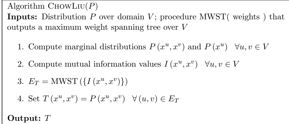
Figure 1: Chow-Liu algorithm (very similar to Meilă and Jordan 2000)
