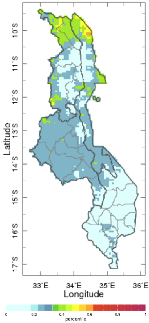
Fig. 1.4: Malawi ENSO Rainfall Forecast Maproom Jan-Mar season, tercile: wet , ENSO state: El Niño
